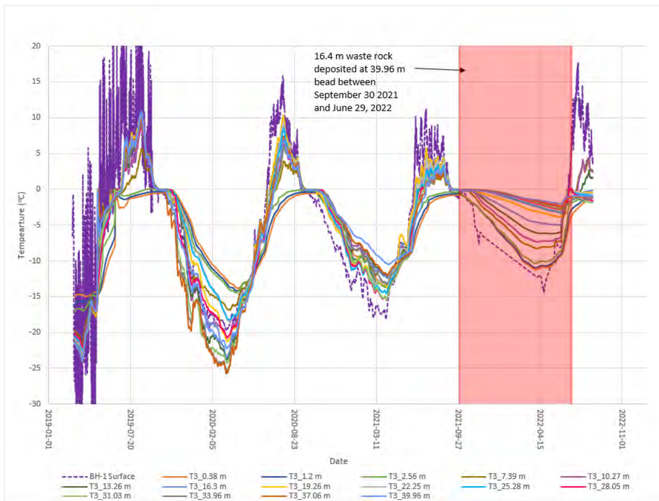
Figure 10: Variation in temperature along T3 from the edge of the pile (0 m) to the end of the string (40 m).
