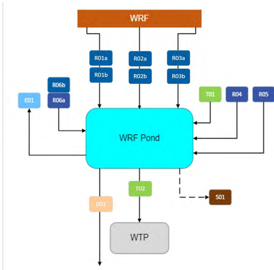
Figure 3: WRF Flow Diagram
