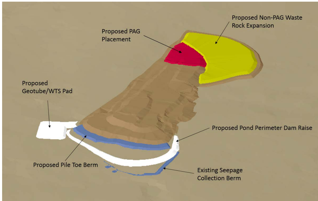
Figure 3: Summer 2018 Waste Rock Deposition Plan– Plan View
