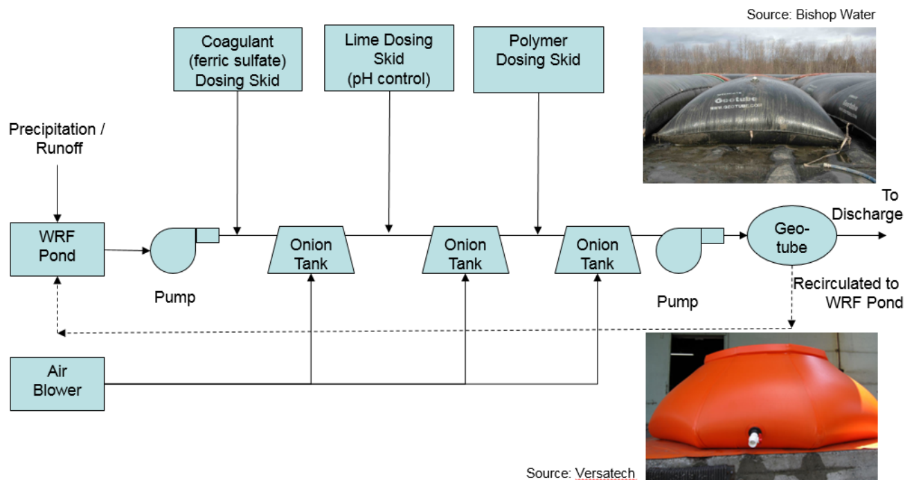
Figure 8: Schematic water treatment flow diagram
