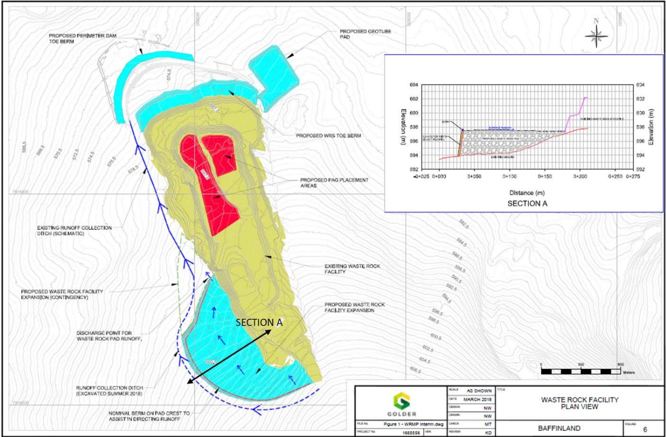
Figure 6: Plan view of temporary water management (Winter 2018).
