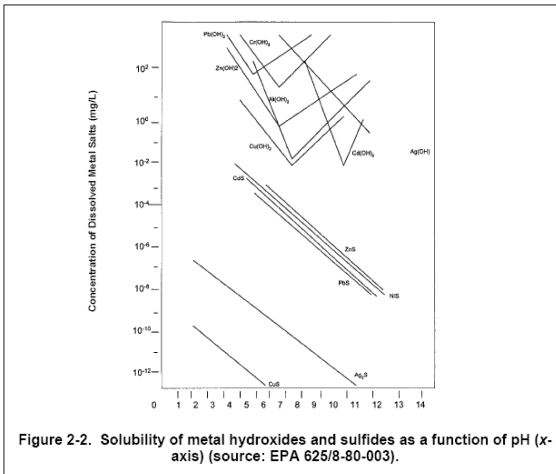
FIGURE 3 SOLUBILITY OF METAL HYDROXIDES AND SULPHIDES
