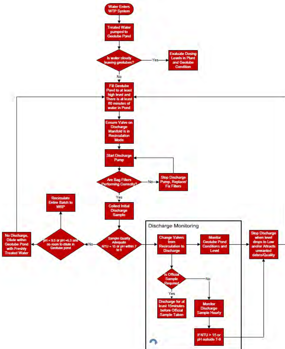
FIGURE 4: WATER TREATMENT PLANT DISCHARGE DECISION FLOWCHART
