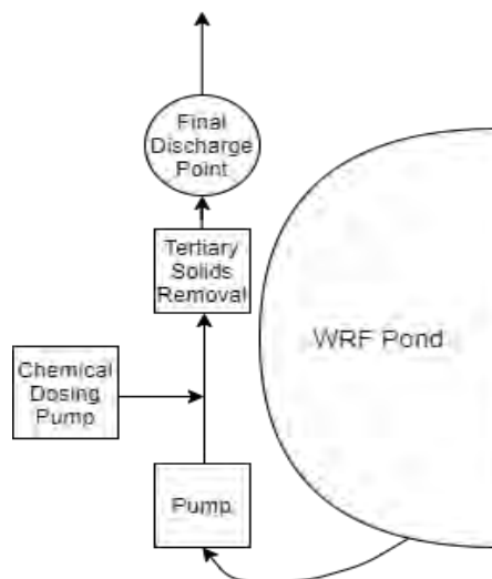
FIGURE 2 TYPICAL DISCHARGE TREATMENT LAYOUT
