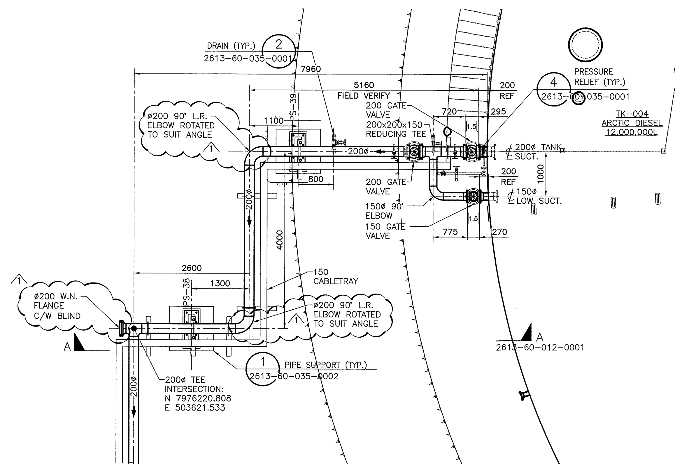
PLAN 1 2613-60-042-0001
