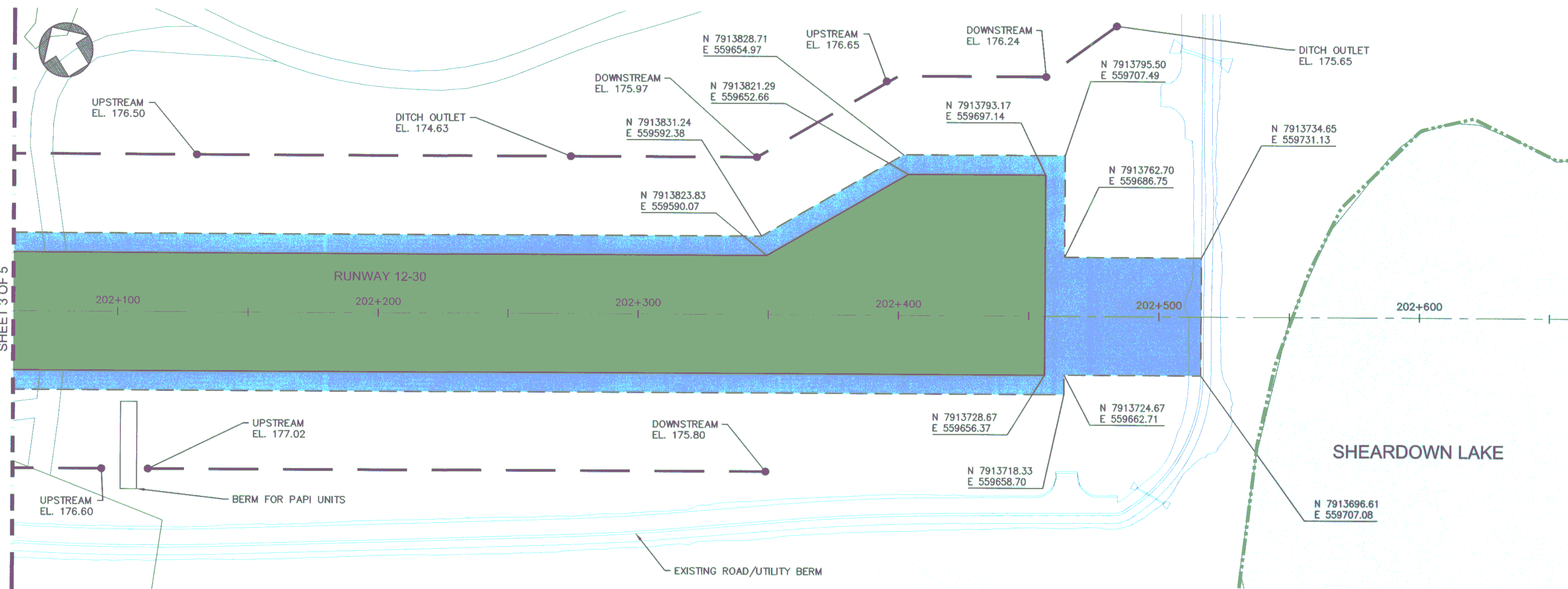
RUNWAY PLAN (STA. 202+060 TO END)
