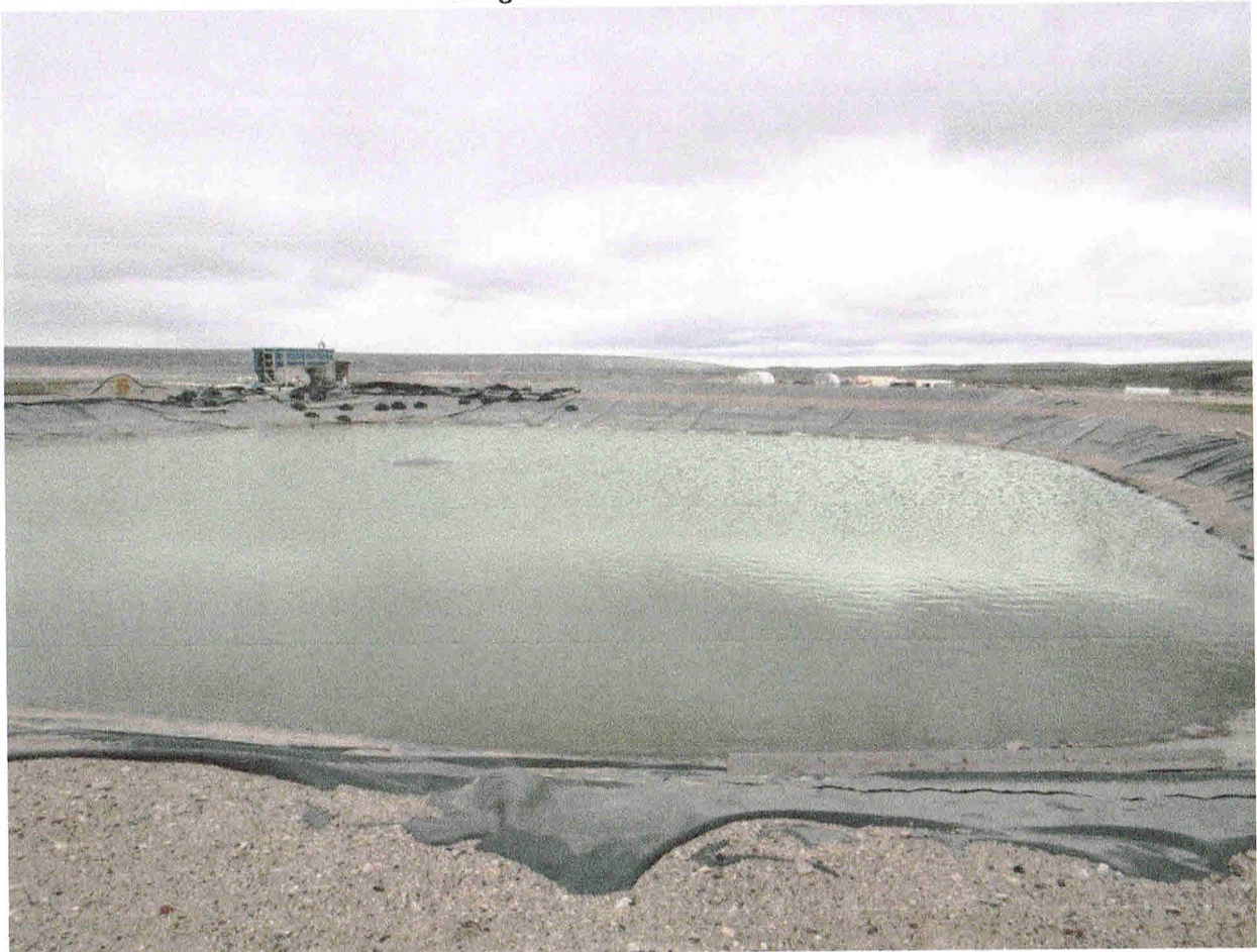
Polishing Waste Stabilization Pond #2.
