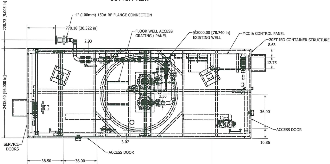
BOTTOM VIEW
