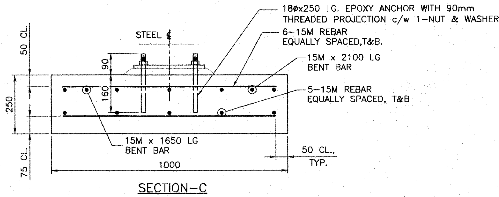
DETAIL PIPE SUPPORTS PS-003 TO 010 SCALE: 1:10
