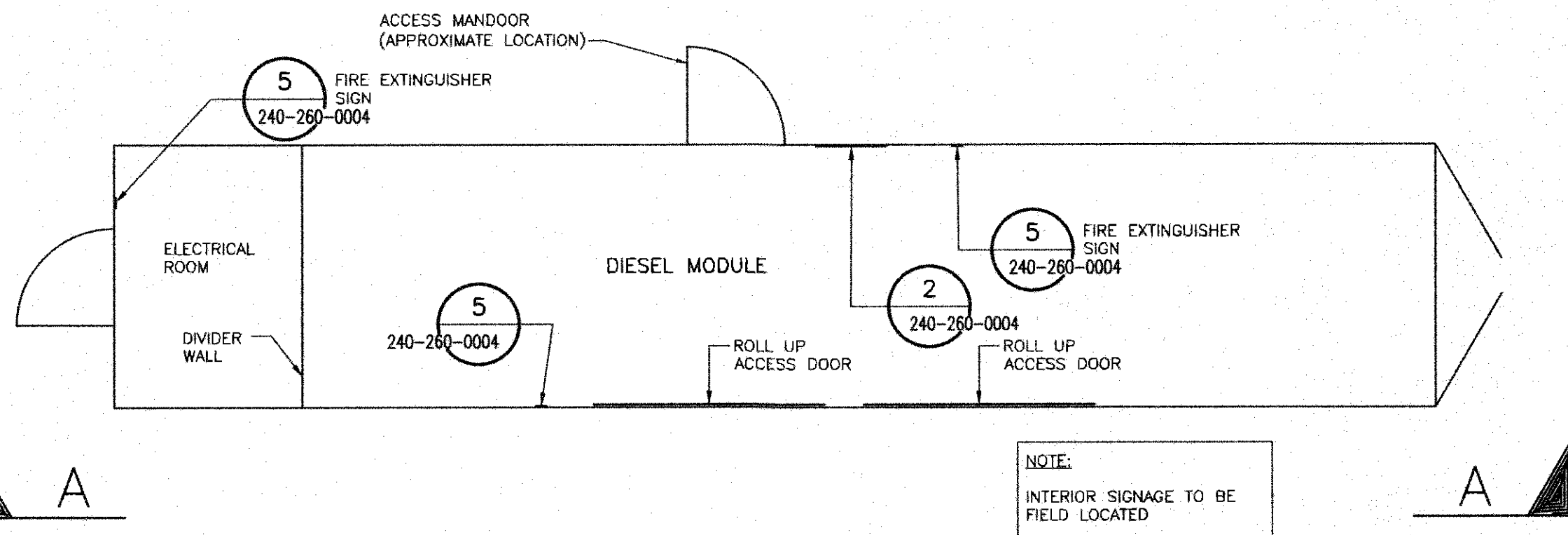
ENLARGED PLAN FUEL MODULE SCALE: 1:50
