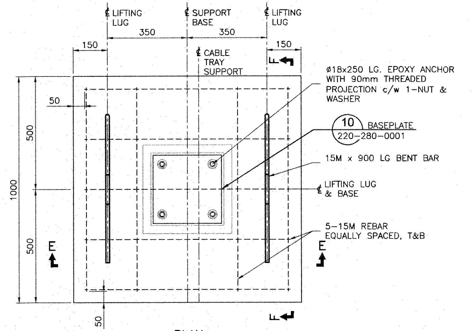
DETAIL CABLE TRAY SUPPORTS CTS-001 TO CTS-002 SCALE: 1:10
