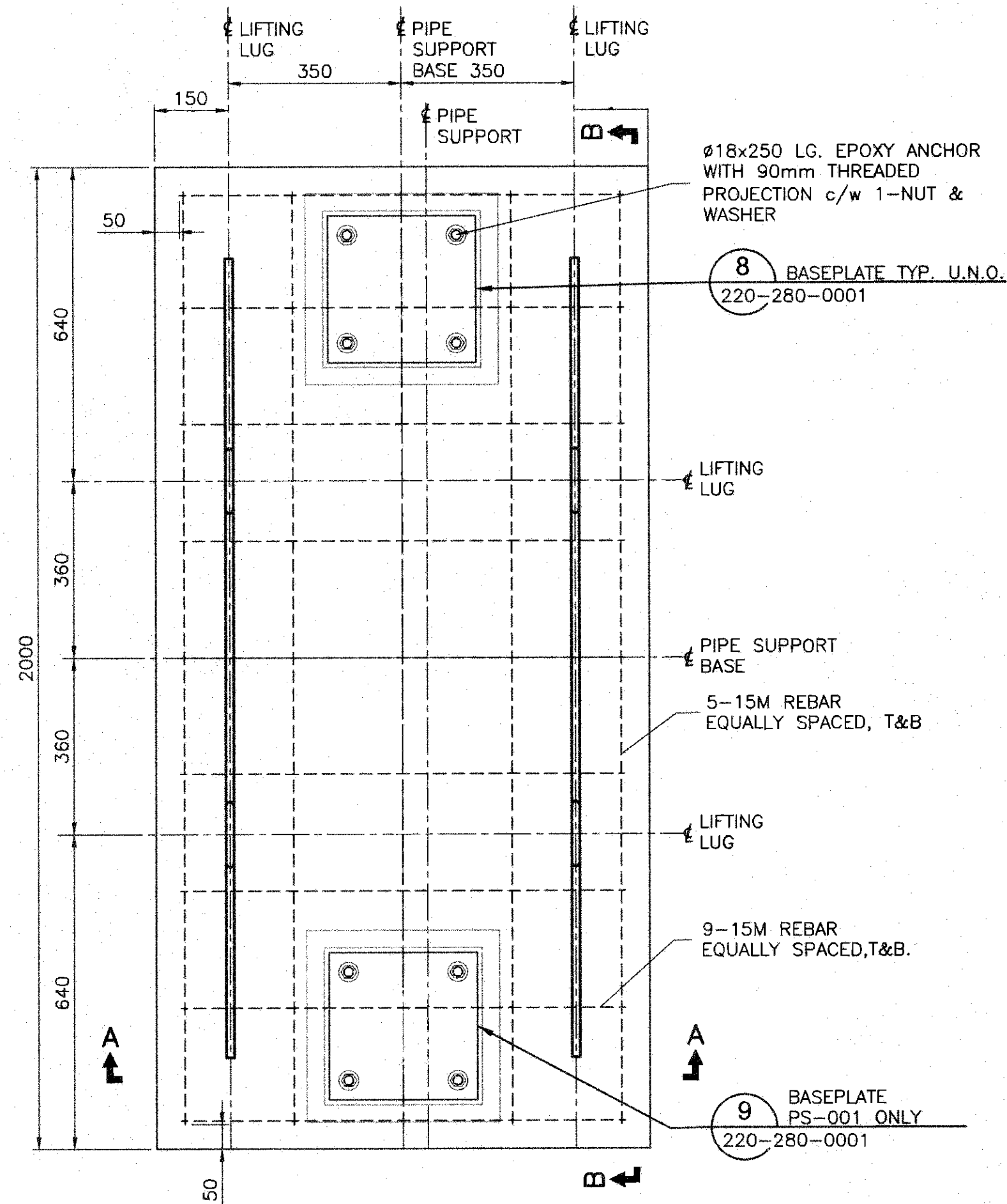
DETAIL PIPE SUPPORTS PS-001, 002, & 011 SCALE: 1:10
