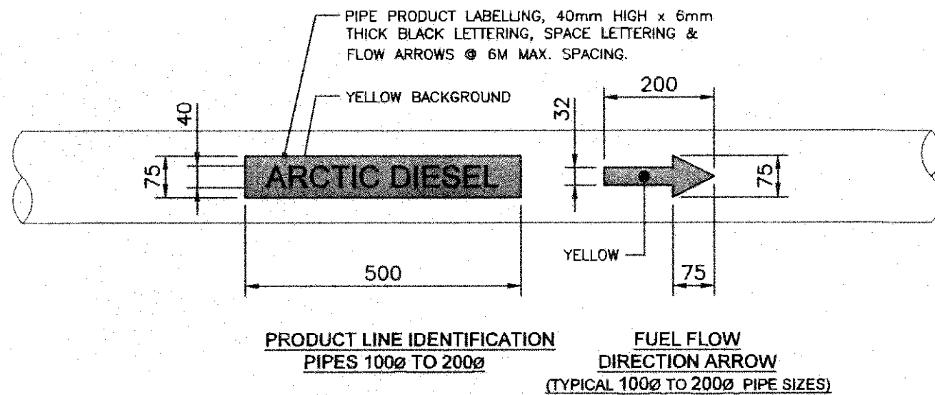
DETAIL PIPE PRODUCT LABELLING SCALE: 1:10
