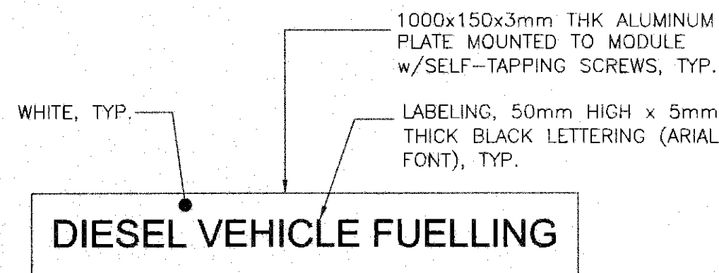
DETAIL DIESEL VEHICLE FUELLING SCALE: 1:10
