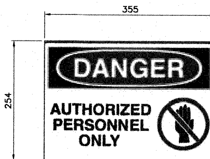
DETAIL 7 AUTHORIZED PERSONNEL SIGN SCALE: 1:5 240-260-0002
