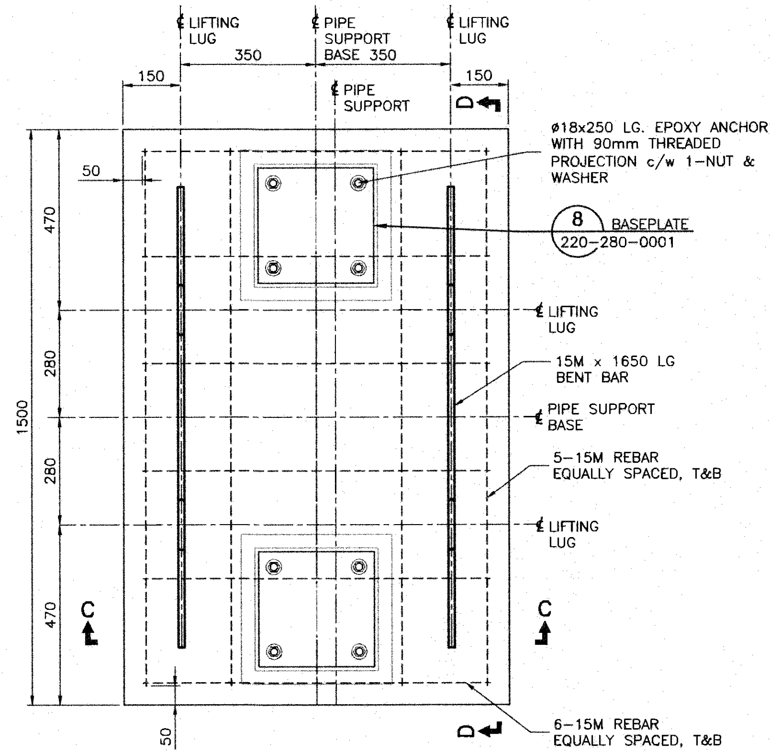
DETAIL PIPE SUPPORTS PS-003 TO 010 SCALE: 1:10
