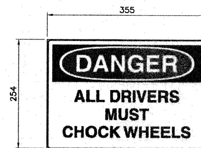
DETAIL 8 CHOCK WHEELS SIGN SCALE: 1:5 240-260-0003
