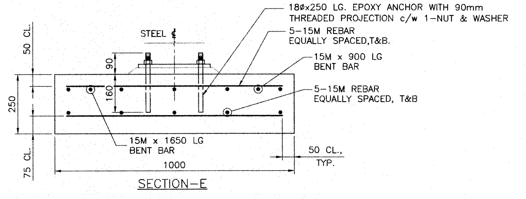
DETAIL CABLE TRAY SUPPORTS CTS-001 TO CTS-002 SCALE: 1:10
