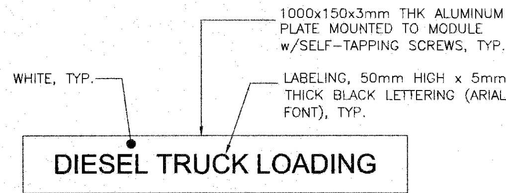
DETAIL DIESEL TRUCK LOADING SCALE: 1:10
