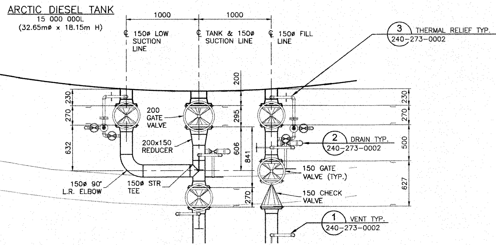
ENLARGED PIPING PLAN DYKE PIPING RACK SCALE: 1:25
