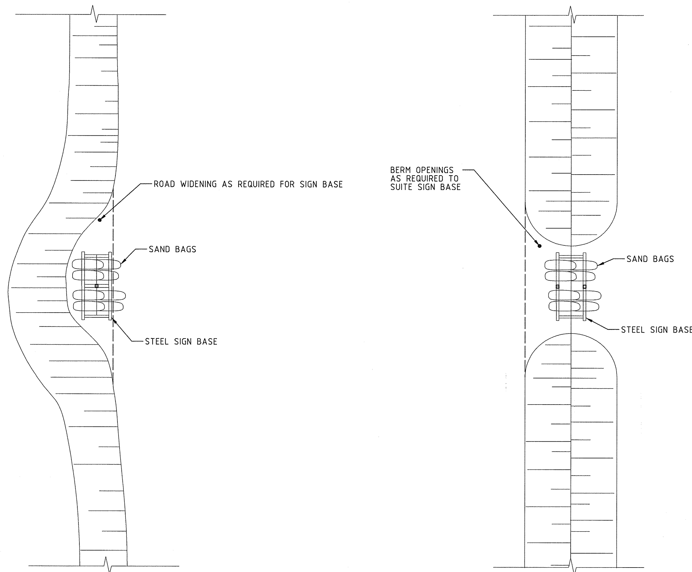
PLAN - PROJECT WIDE SIGN PLACEMENT CONFIGURATION N.T.S.
