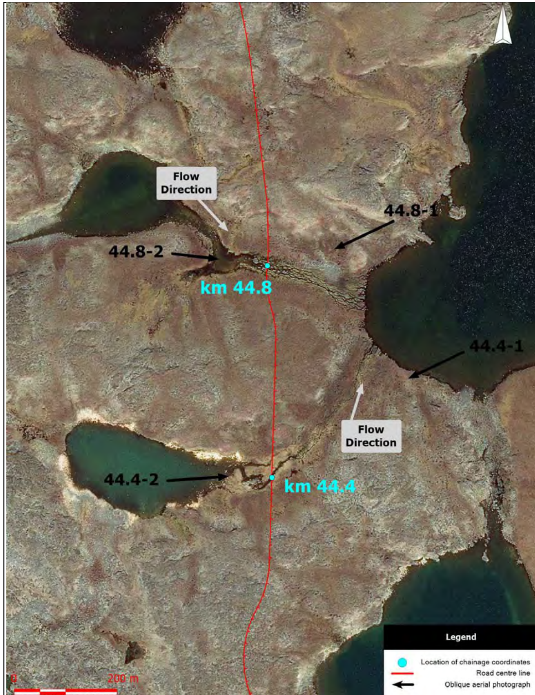
Kilometres 44.4 and 44.8. Aerial photograph showing the road centre line, the location of chainage coordinates provided in Table 3-2, the flow direction, and the location of oblique aerial photographs.
