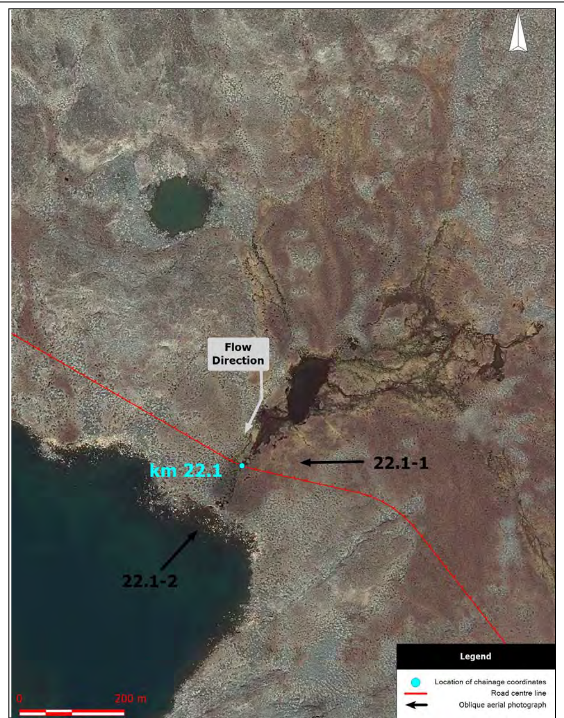
Kilometre 22.1. Aerial photograph showing the road centre line, the location of chainage coordinates provided in Table 3-2, the flow direction, and the location of oblique aerial photographs.
