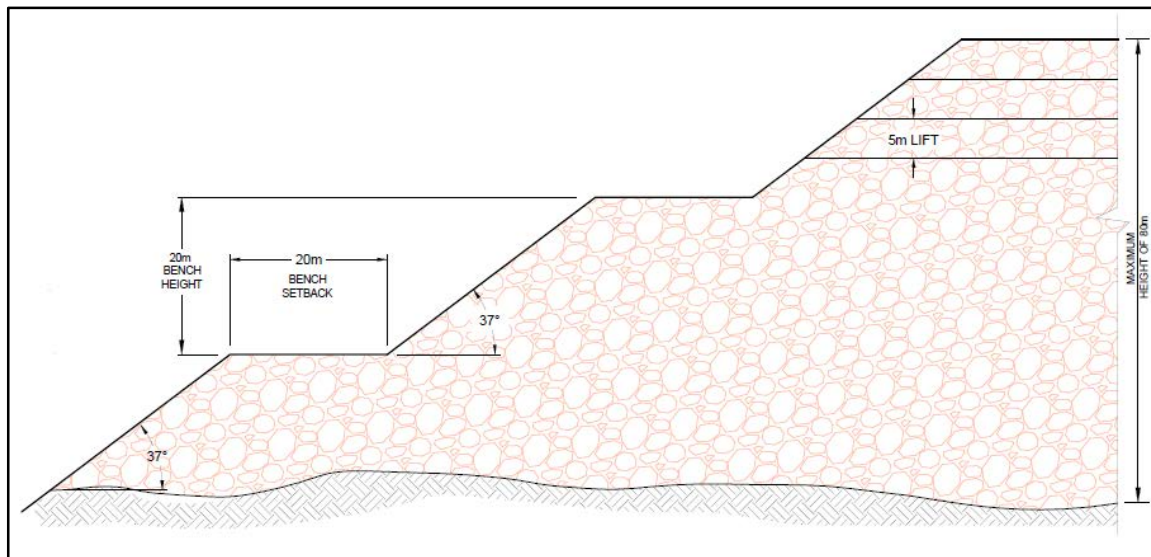
Figure 6.4 Typical Cross Section of the Whale Tail Waste Rock Storage Facility
