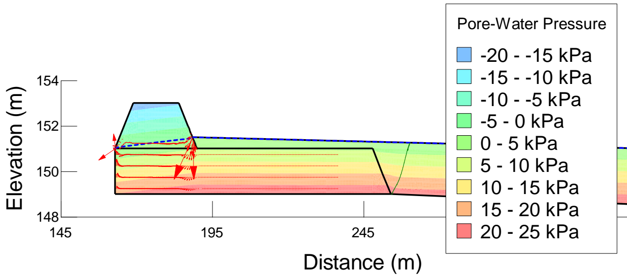
Figure 20: Steady-state pore-water pressure, flow paths and flow vectors for section 5 at end of 2020
