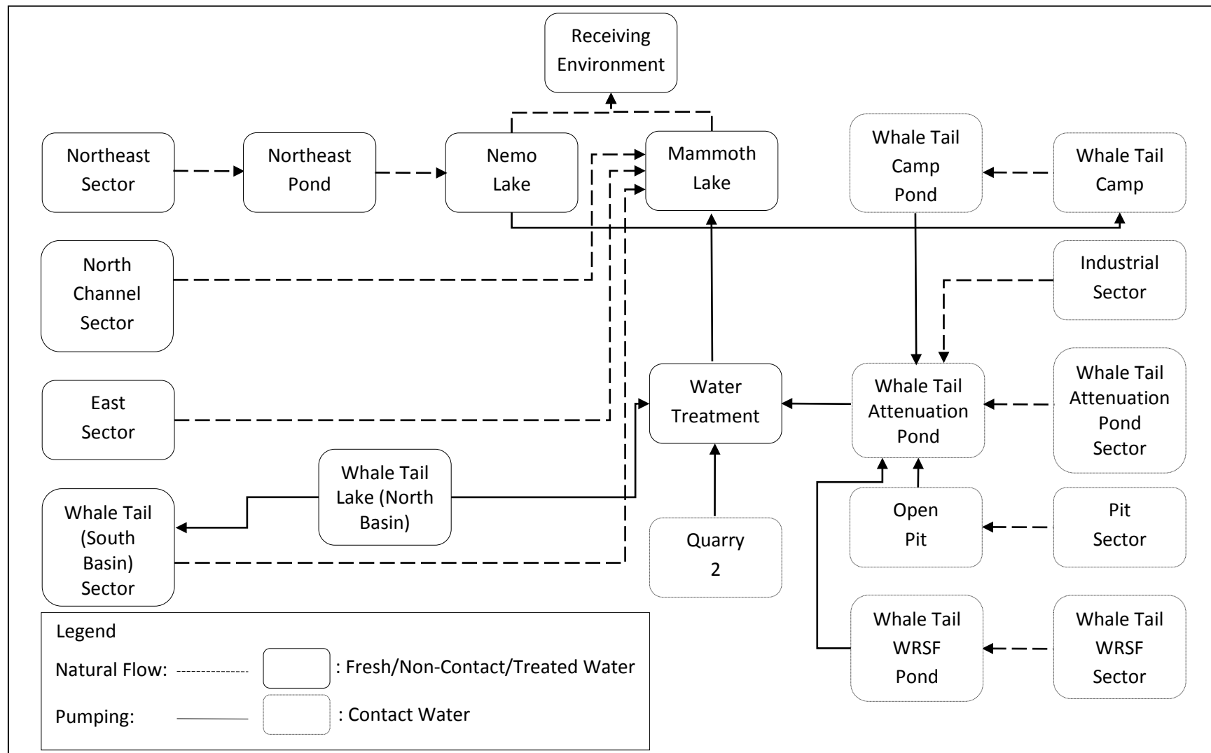
Figure B.1 Water Management Flowsheet during Construction and Operations
