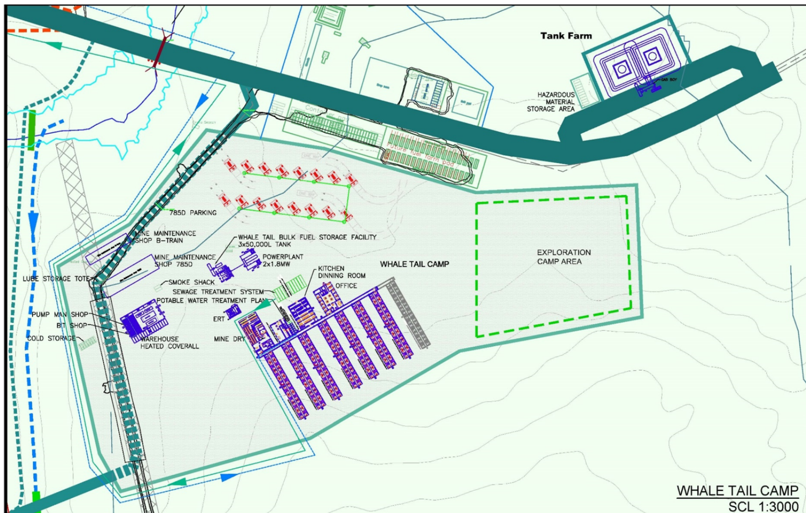
Figure 5. Layout Whale Tail Open Pit camp
