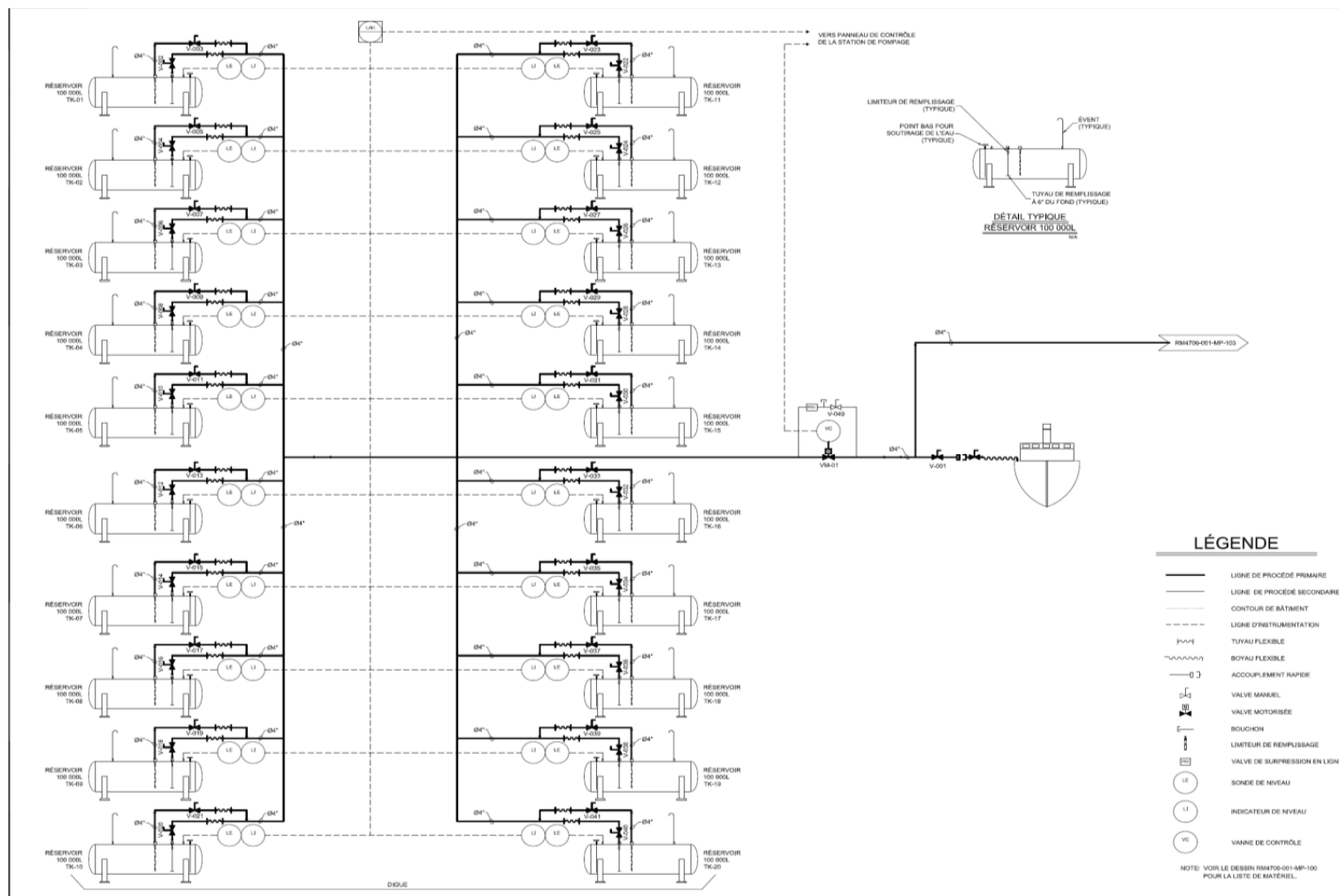
Figure 4 : Baker Lake Jet-A Fuel Tank Farm
