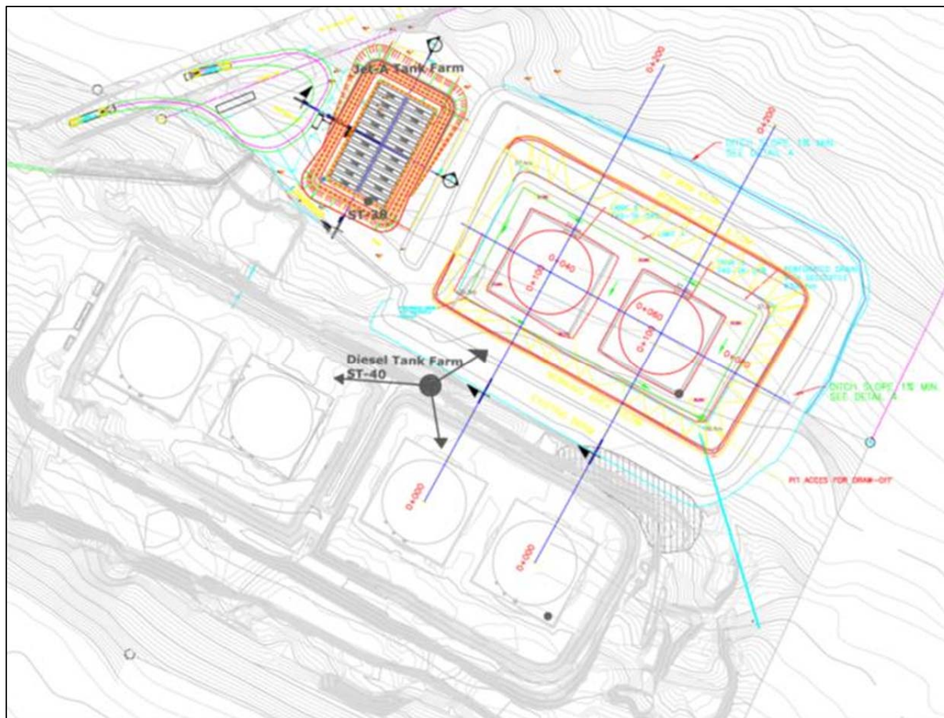
Figure 3 : Baker Lake Diesel Fuel Tank Farm
