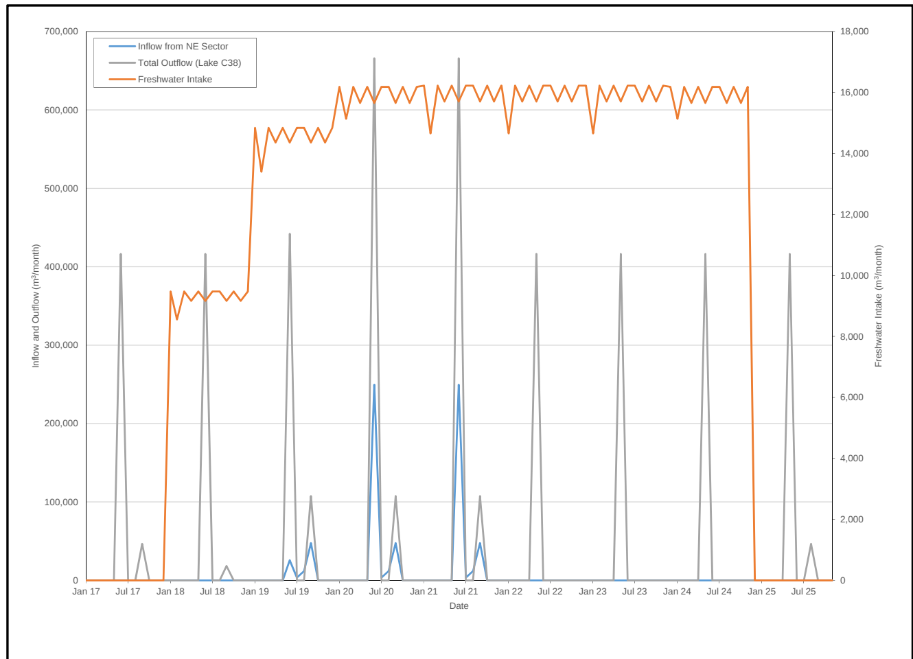
Figure 1: Lake C38 (Nemo Lake) Water Balance from 2017 to 2025
