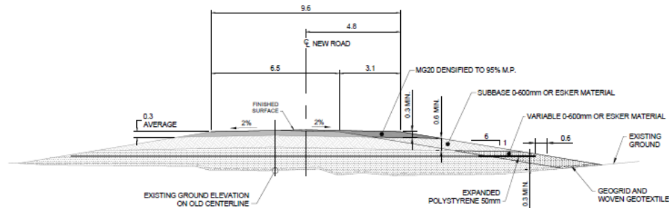
TYPICAL SECTION 5 ICE WEDGE AND VERY THAW SUSCEPTIBLE SOIL (SEE NOTE 1)
