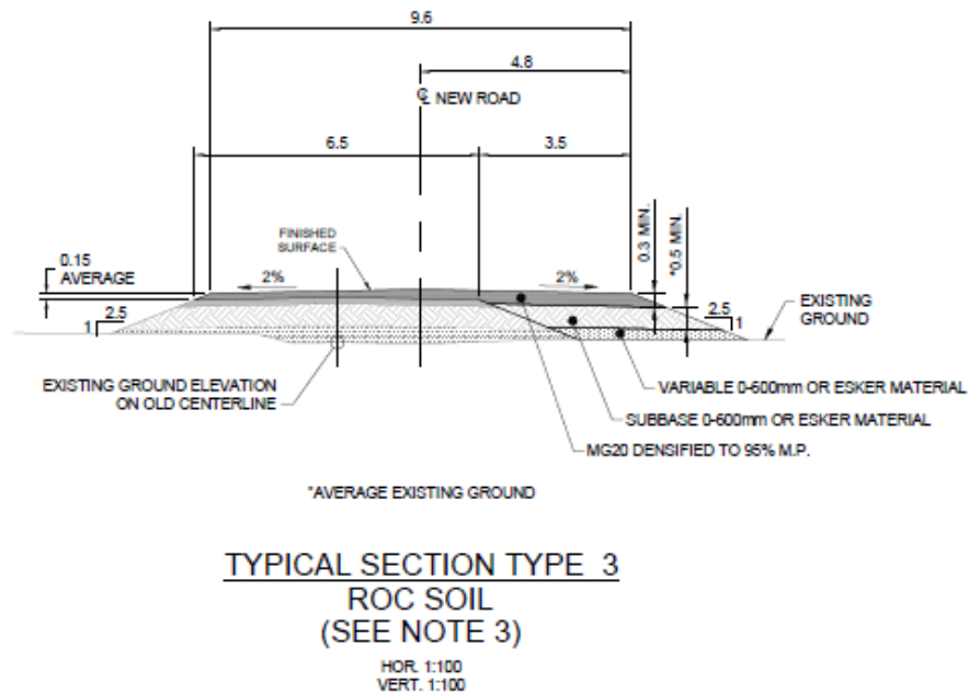
Figure 5.3 Typical section of Haul road built over soil relatively unsuceptible to freeze and thaw settlement
