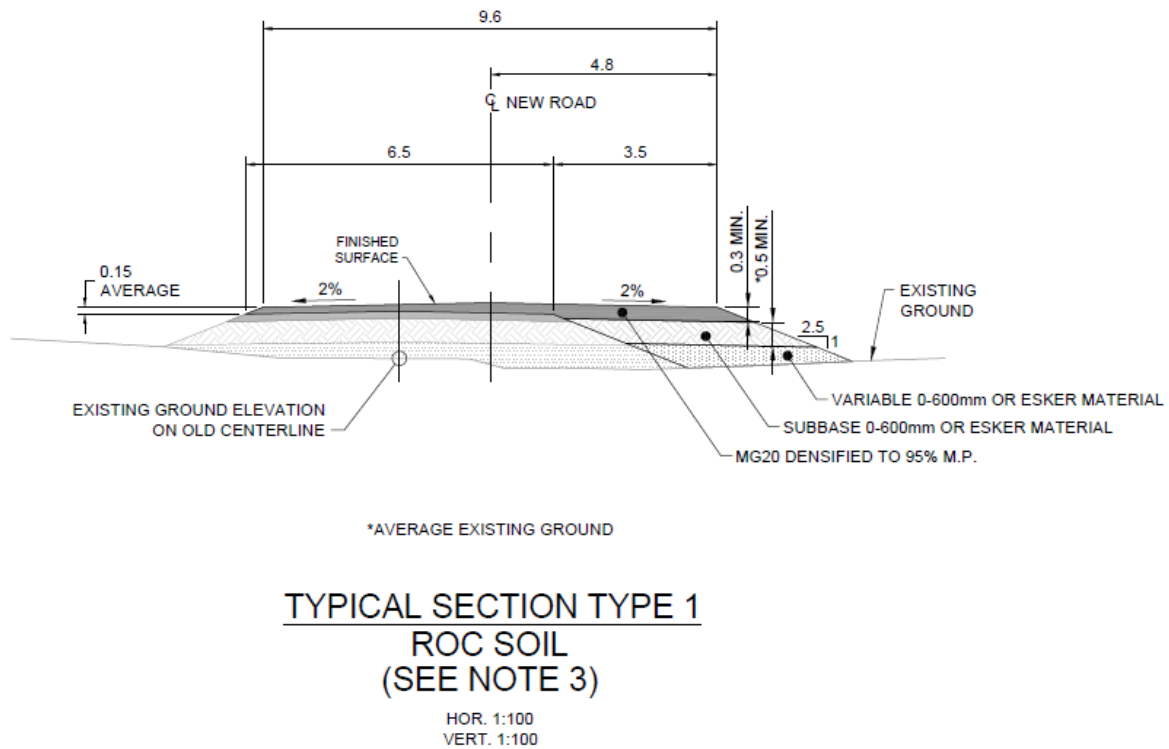
Figure 1.1. Cross section view of the expanded Whale Tail Pit Haul Road
