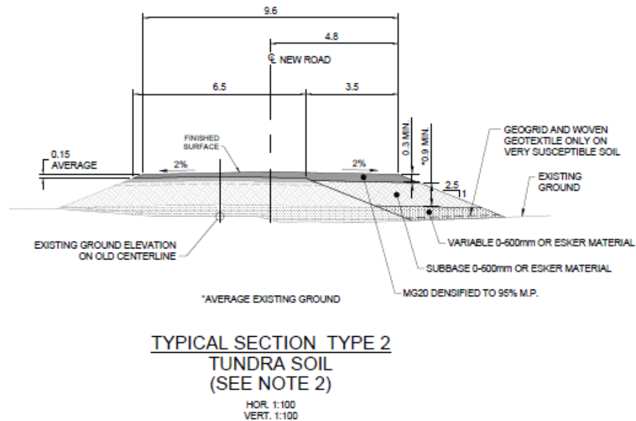
Figure 5.2 Typical Cross-section of Haul road built over thaw susceptible soil
