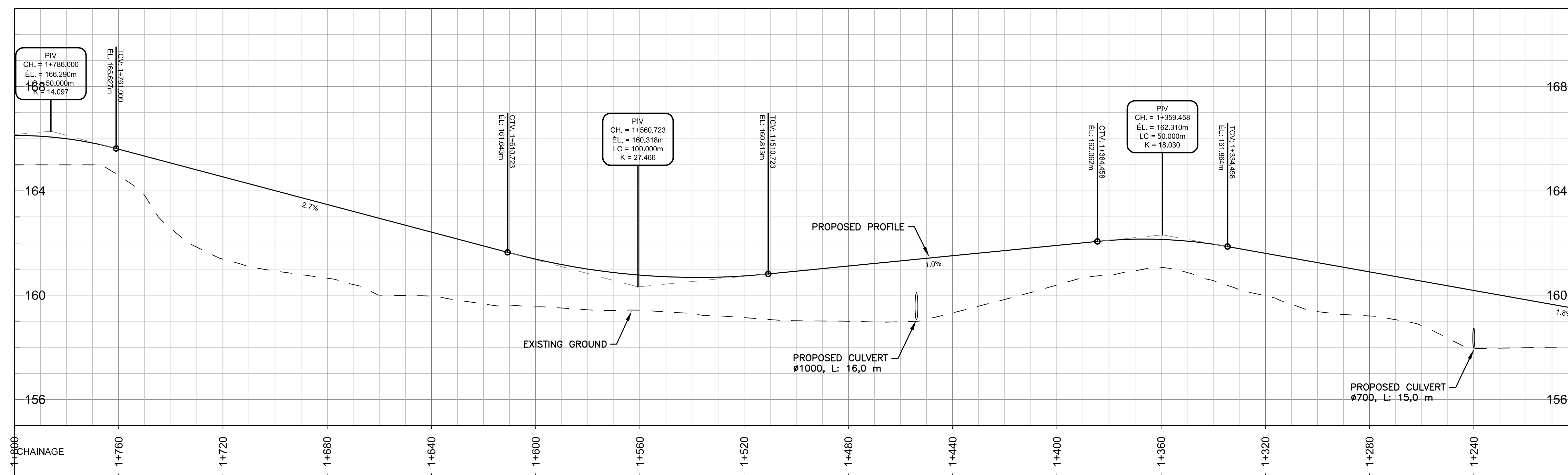
ROAD #22 - EXPLOSIVE ROAD SCALE : 1:1000
