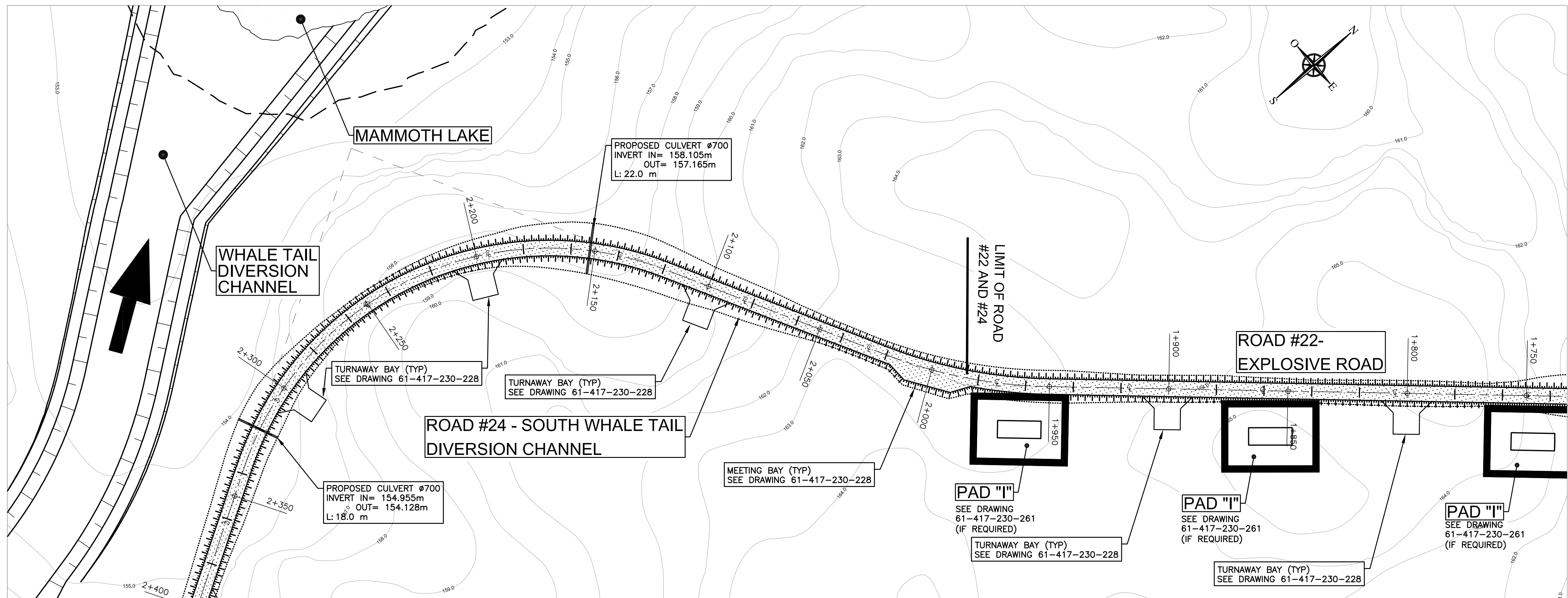
ROAD #22 AND ROAD #24 SCALE : 1:1000
