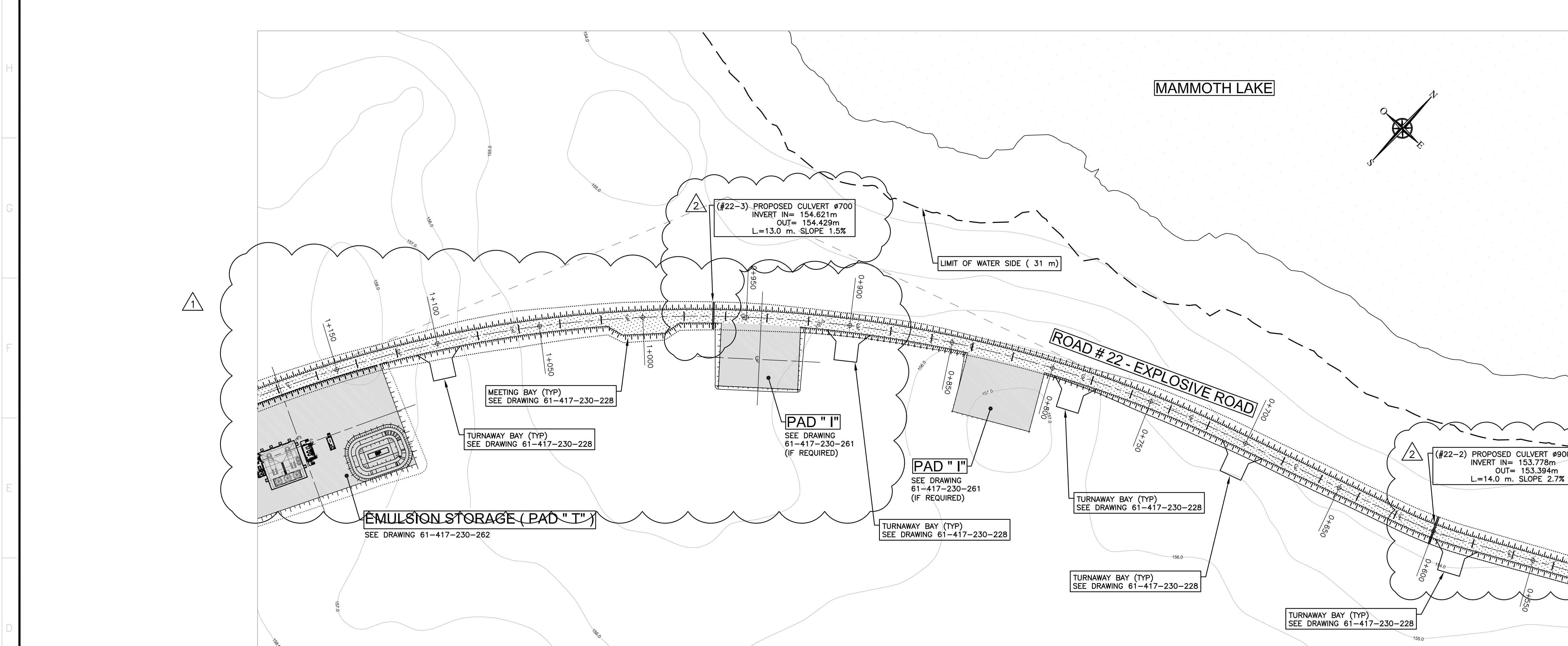
ROAD #22 - EXPLOSIVE ROAD SCALE : 1:1000
