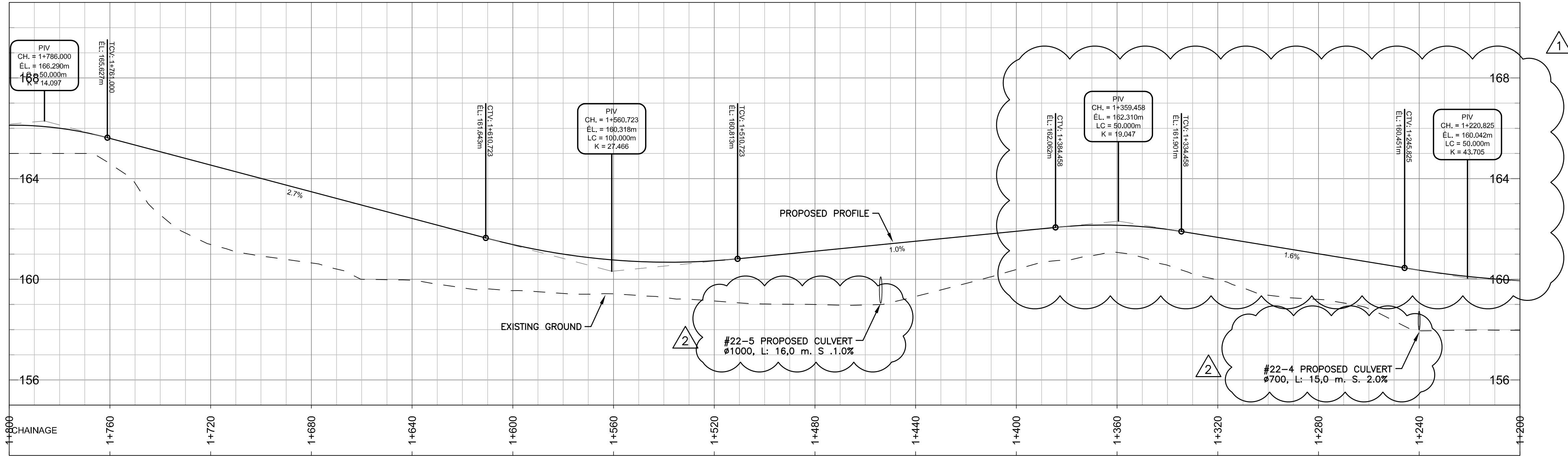
ROAD #22 - EXPLOSIVE ROAD SCALE : 1:1000
