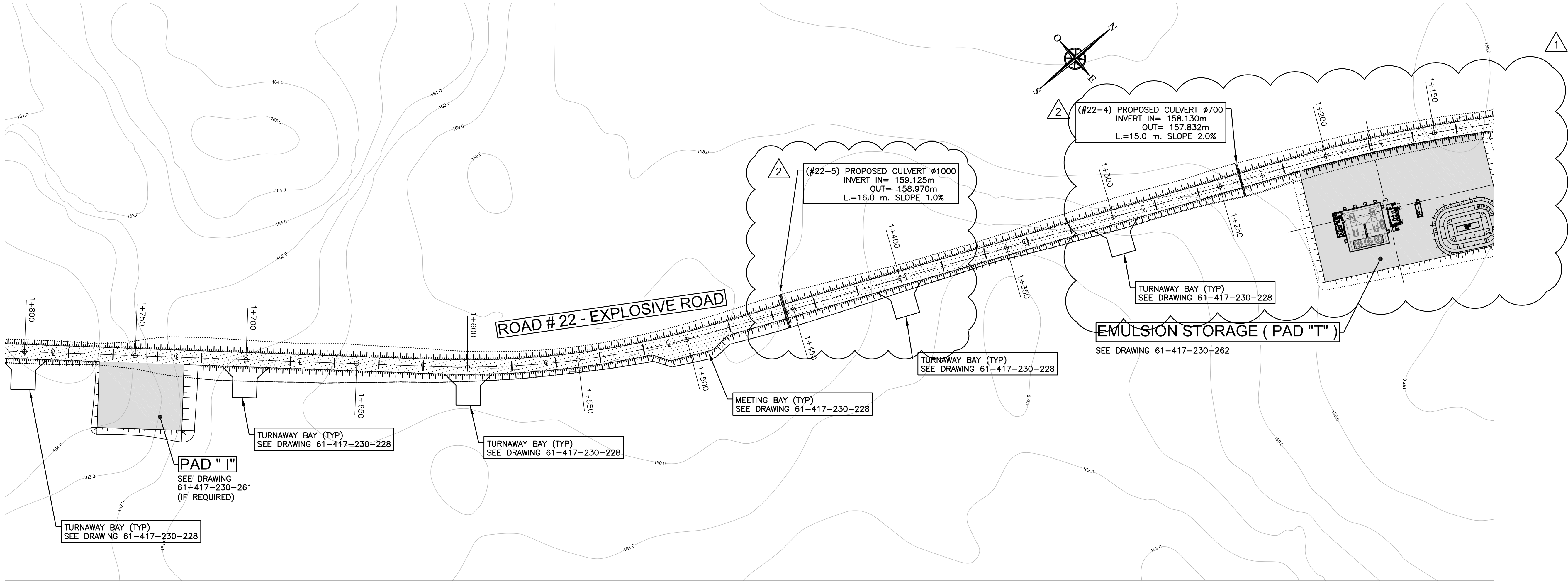
ROAD #22 - EXPLOSIVE ROAD SCALE : 1:1000
