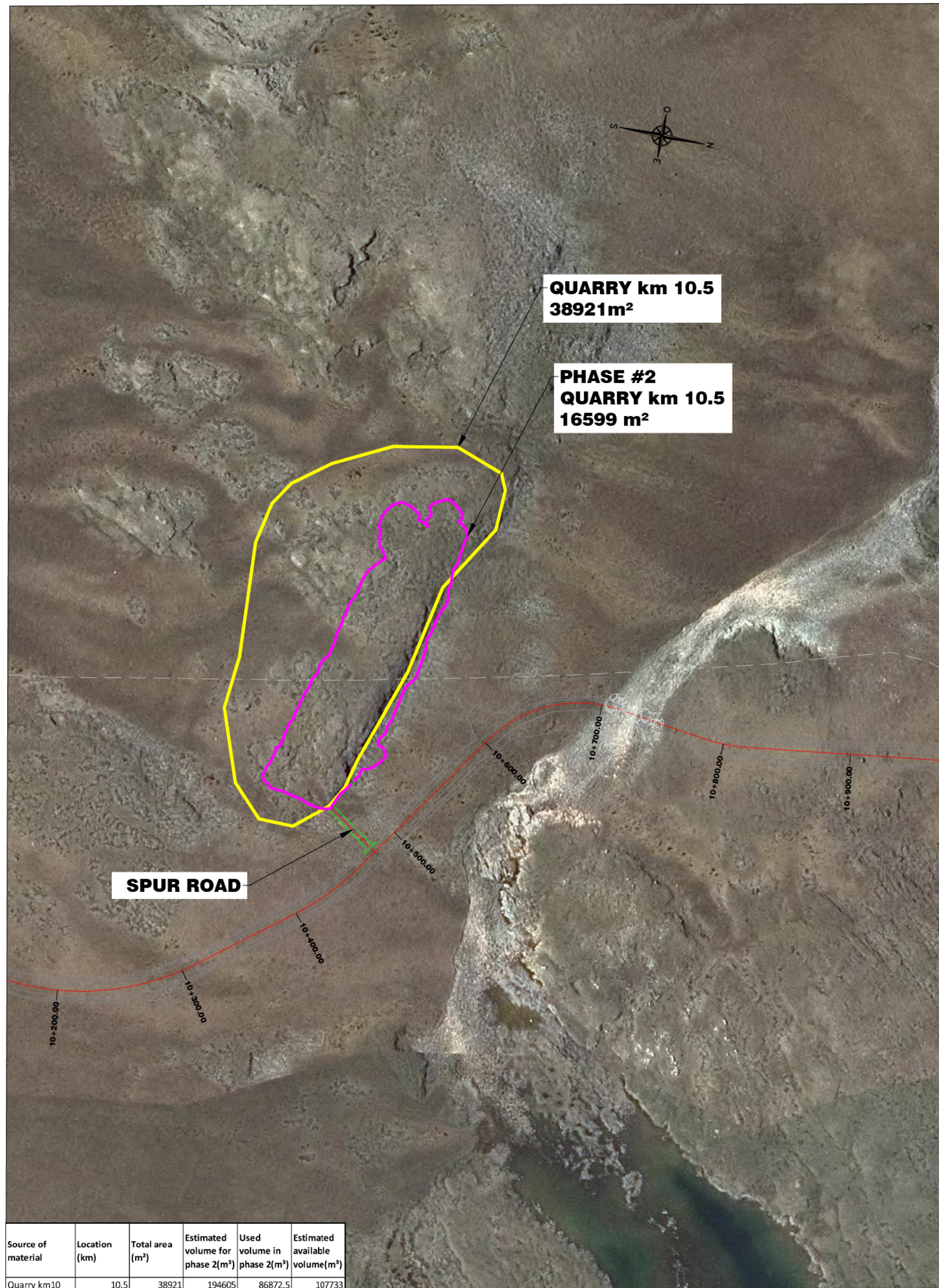
PLAN QUARRY KM 10.5 ÉCH :1 :2000
