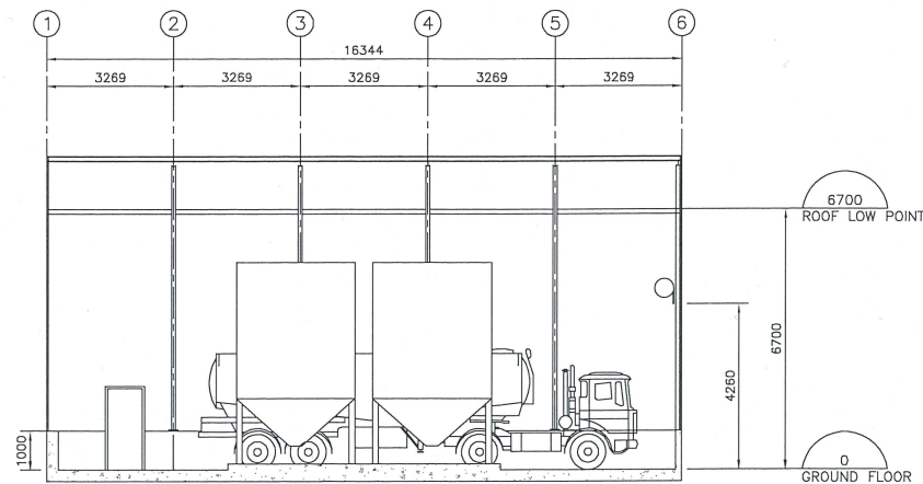
SECTION A 1:100
