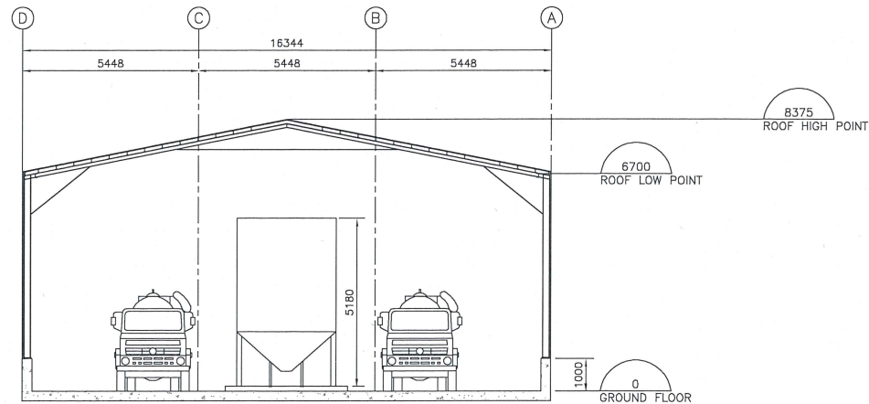
SECTION B 1:100
