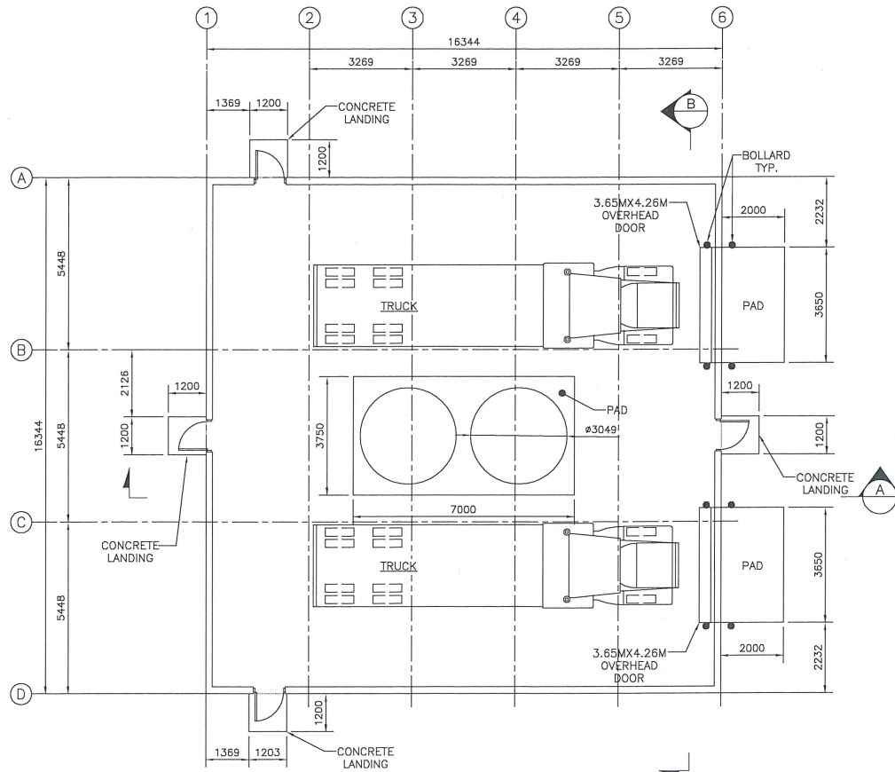
EMULSION PLANT MAIN FLOOR 1:100
