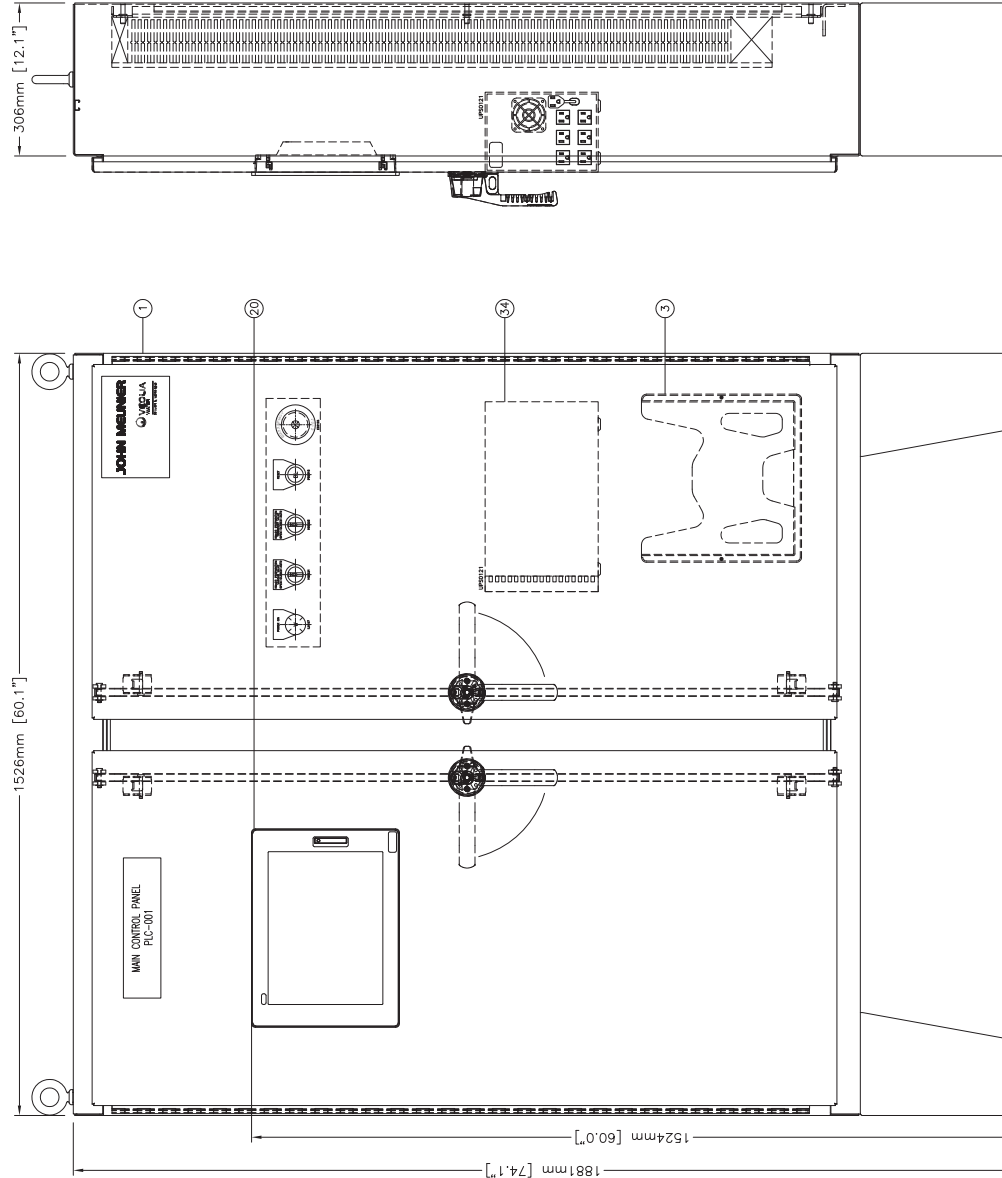
SIDE LAYOUT
