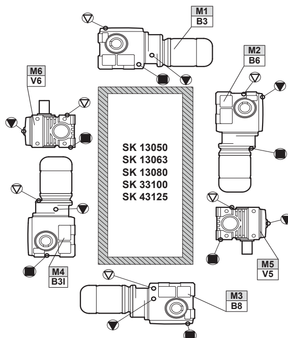
Foot Mount
