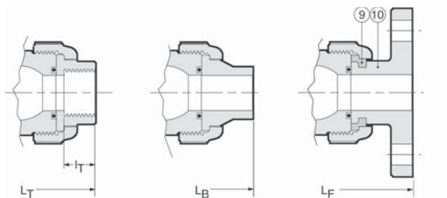
NPT Threaded
