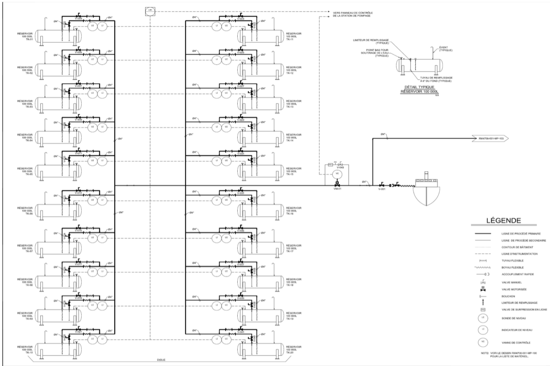
Figure 4 : Baker Lake Jet-A Fuel Tank Farm
