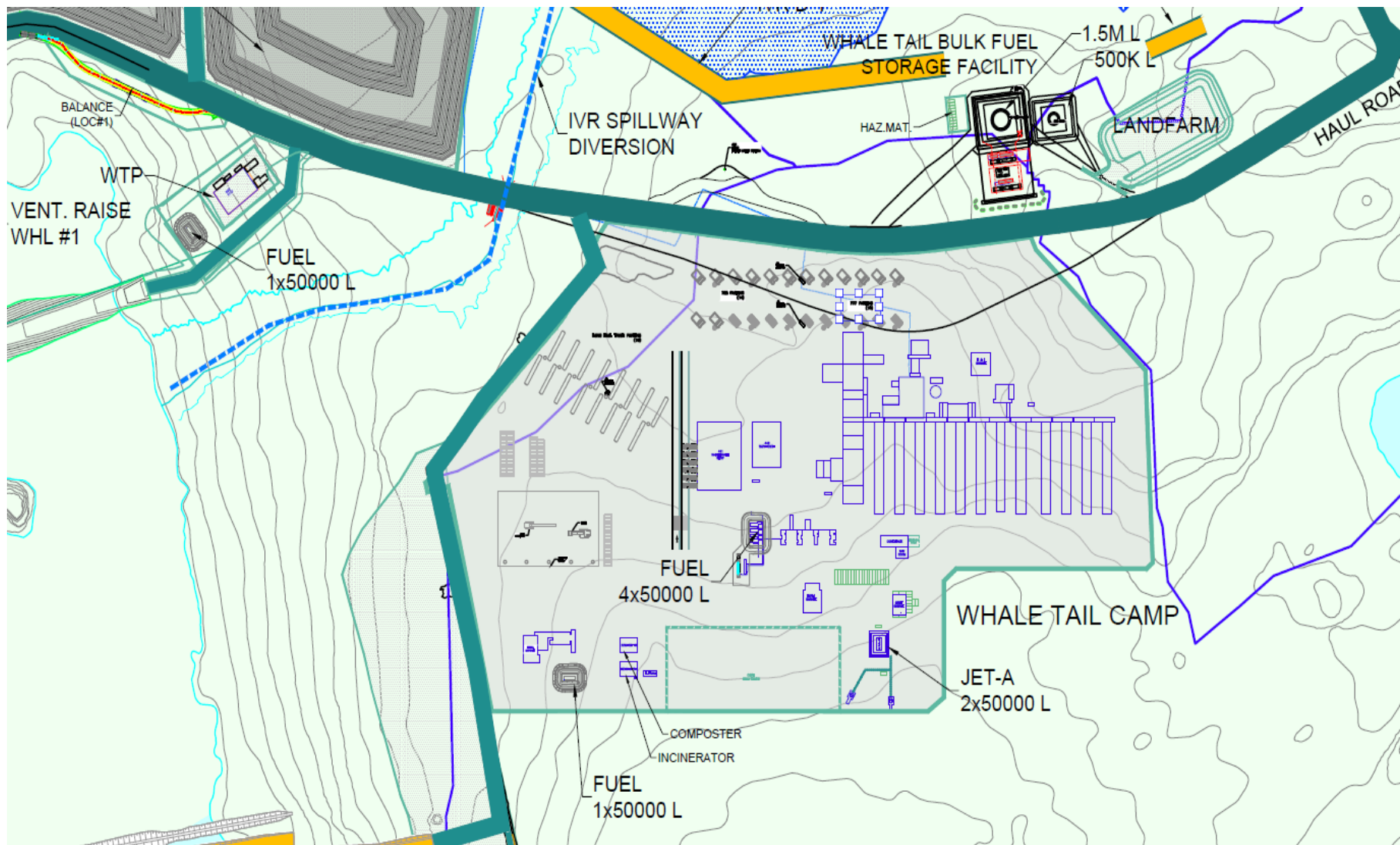
Figure 5. Layout Whale Tail Pit Expansion Project Camp
