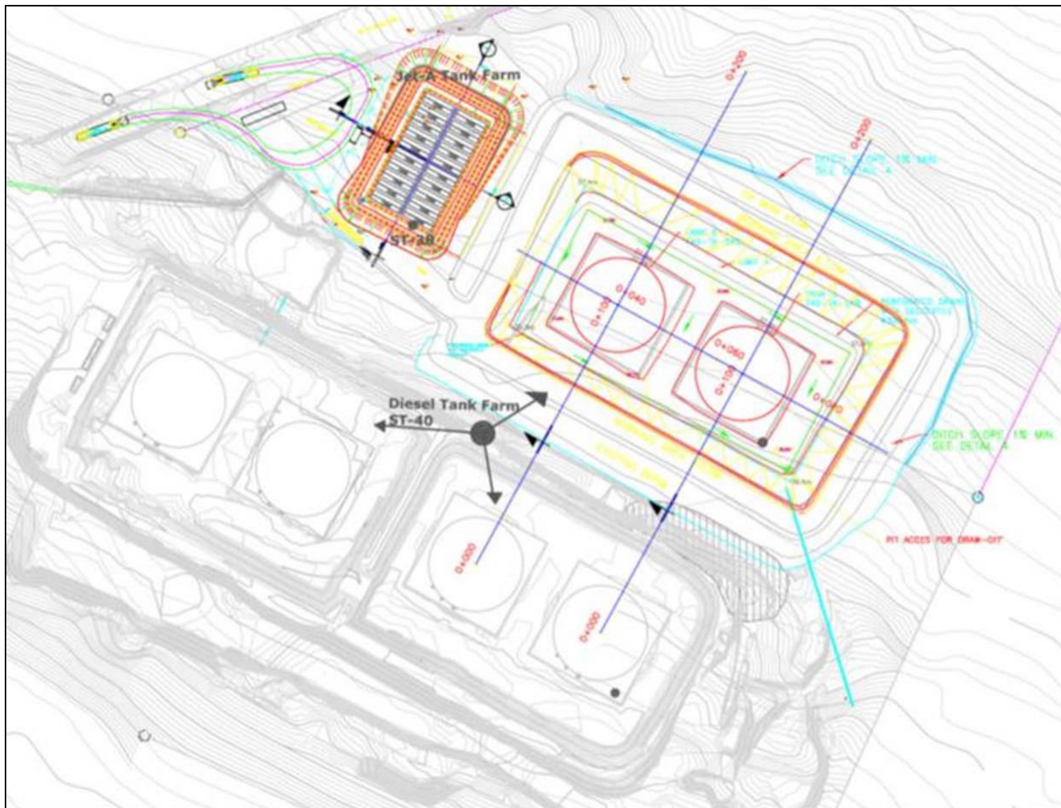
Figure 3: Baker Lake Diesel Fuel Tank Farm
