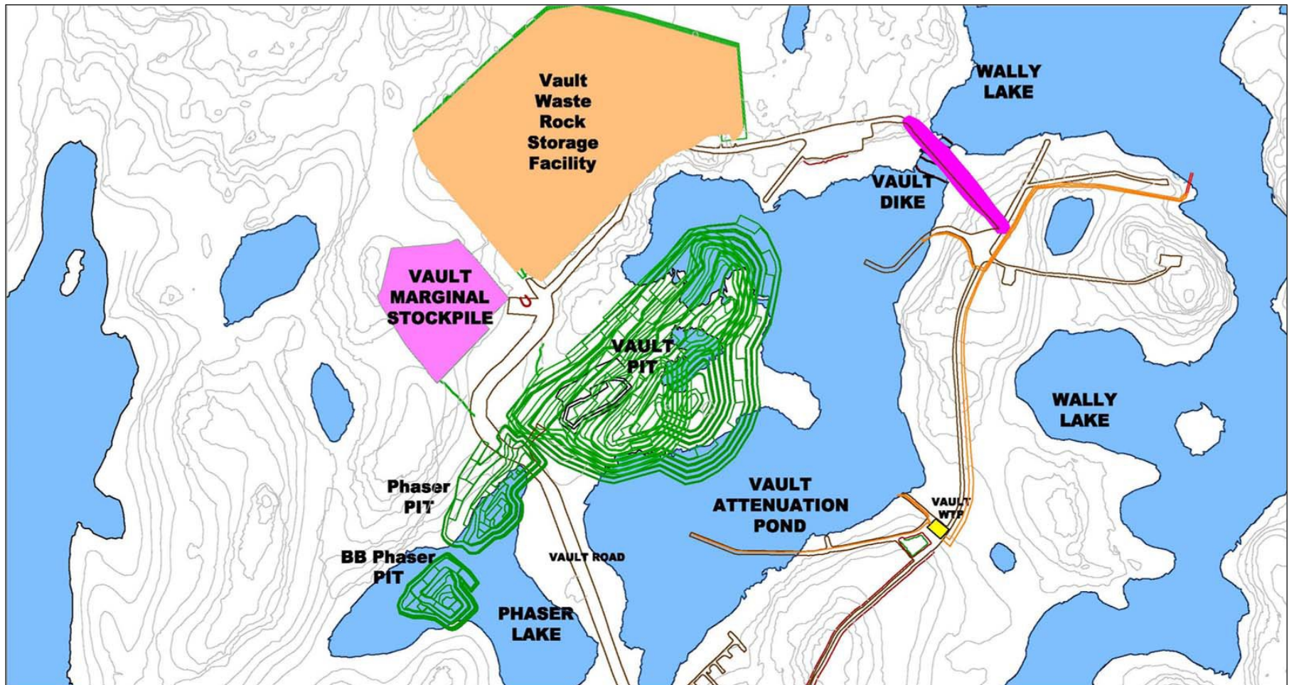
Figure 2 : Layout Vault
