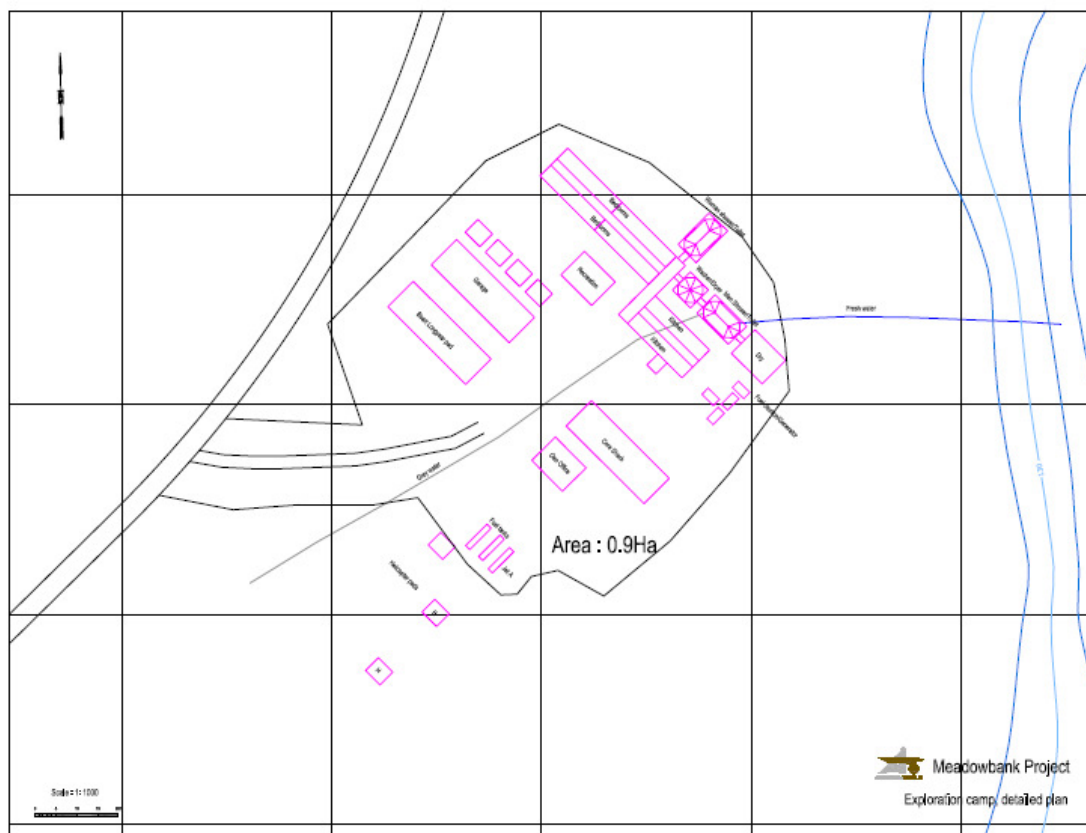
Figure 2.2: General layout of camp
