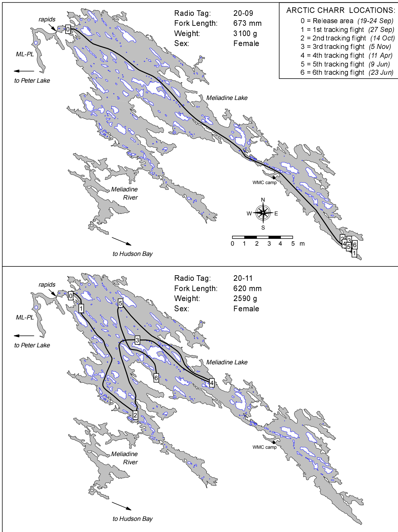
Appendix F26. Movements of radio tagged Arctic Char in the Meliadine Study Area, Sept 2000 to Jun 2001.
