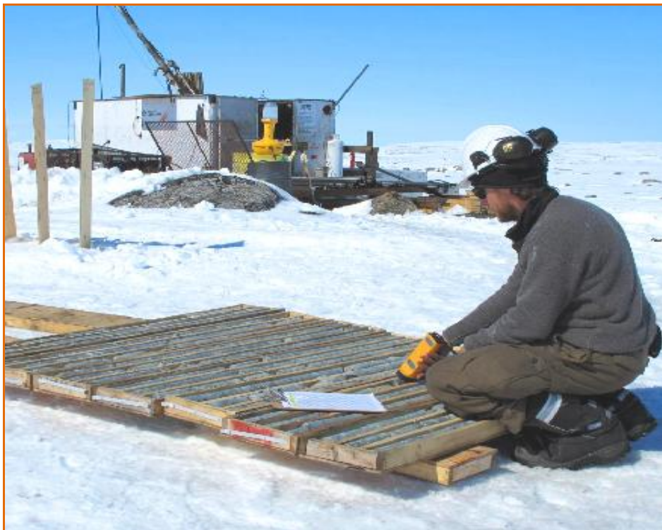
TOP: Northspan Hornet waterless reverse-circulation drill in operation at QLQ-28 – July 2011; 40 RC holes in total, producing chips rather than core, were drilled between 11 May-07 September 2011. ABOVE: Core drilling at CH-55 kimberlite – May 2011.
