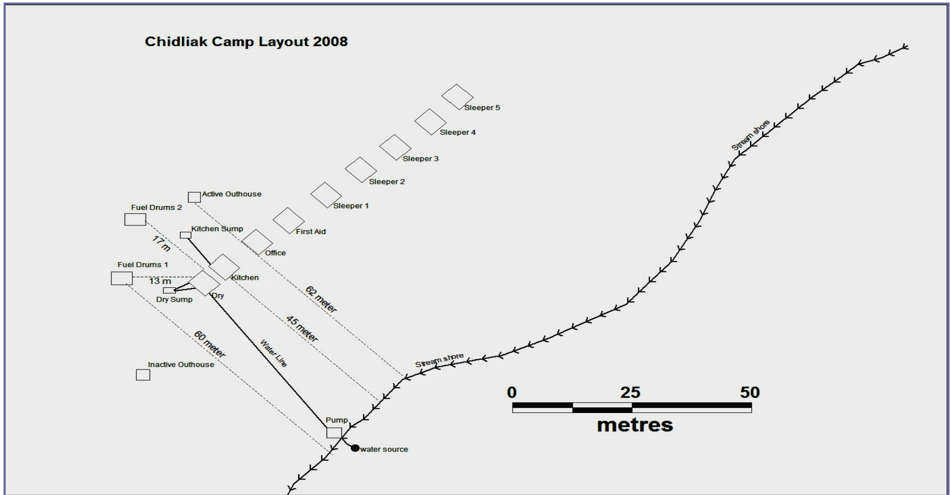
Figure 3: Chidliak Camp Site Map (NTS 26B/01)
