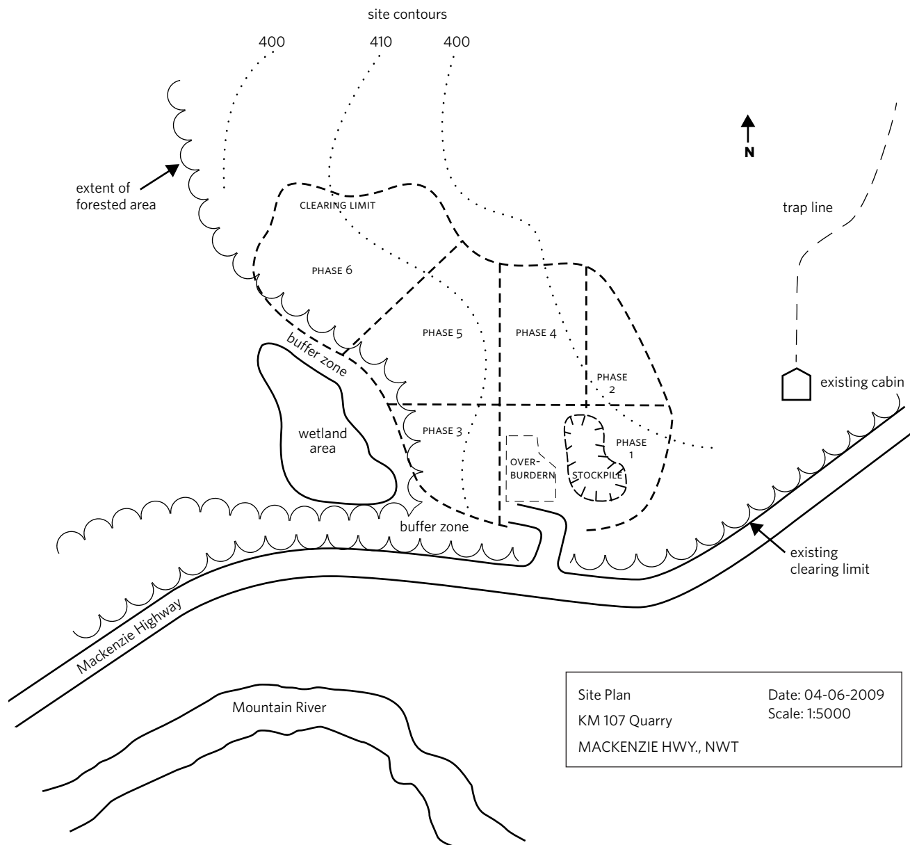
FIGURE 15. Site design diagram to be submitted with a pit/quarry development plan. (Redrawn from Robertson and Brandt, 1997, p. 64.)
