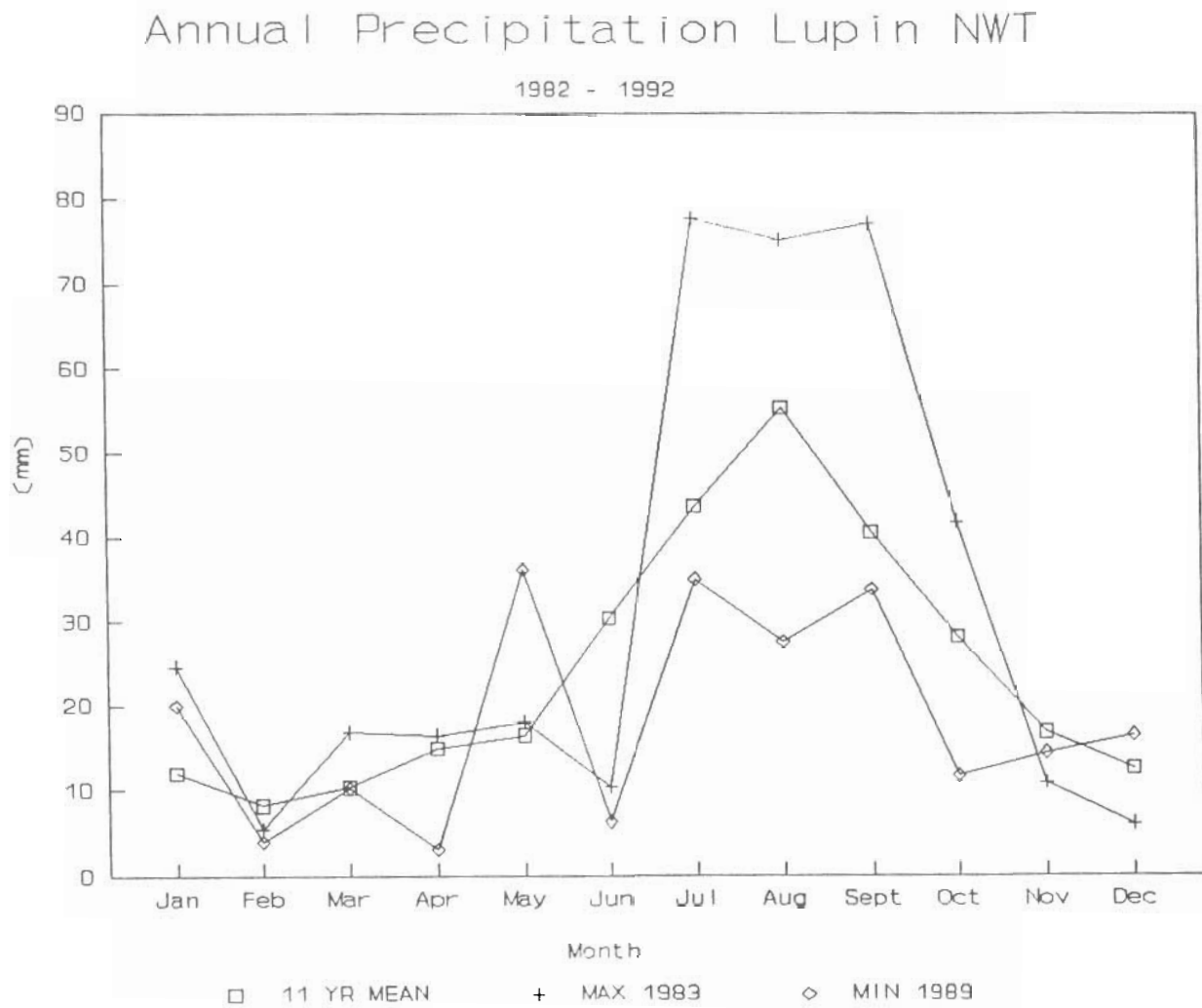
Figure 13: Annual precipitation for Lupin AES Station, NWT (1978-1993).
