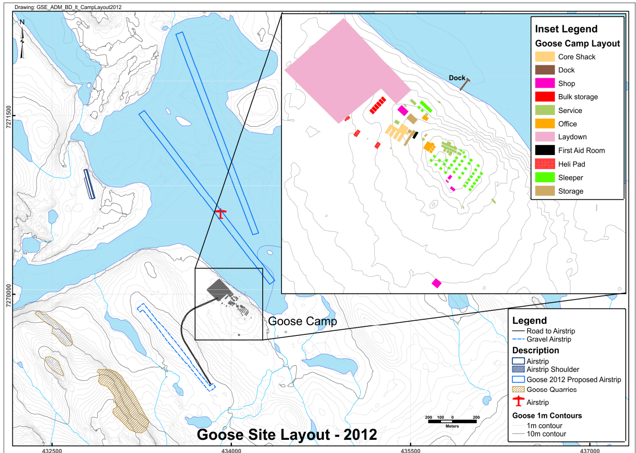
Figure 3. Goose camp site layout
