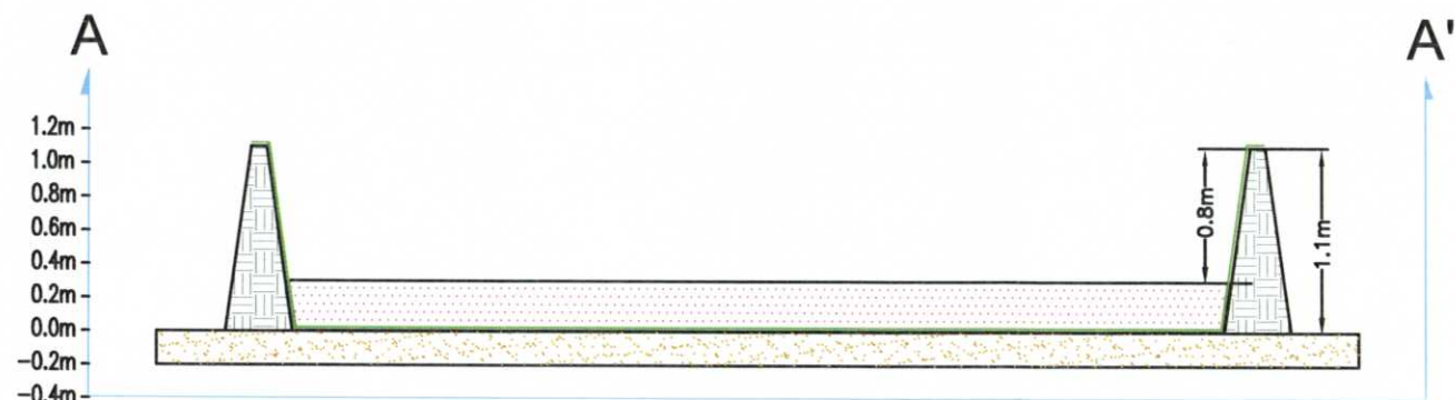
CROSS-SECTION A-A' Vertical Exaggeration : 5X
