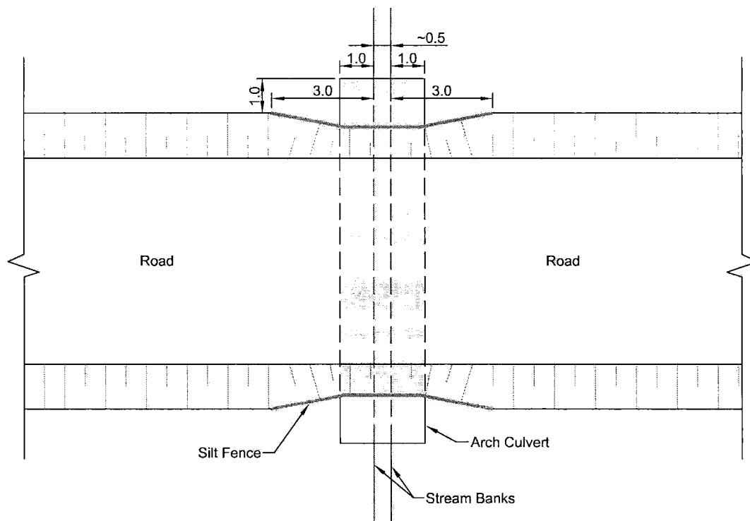
Plan View - After Culvert Installation
