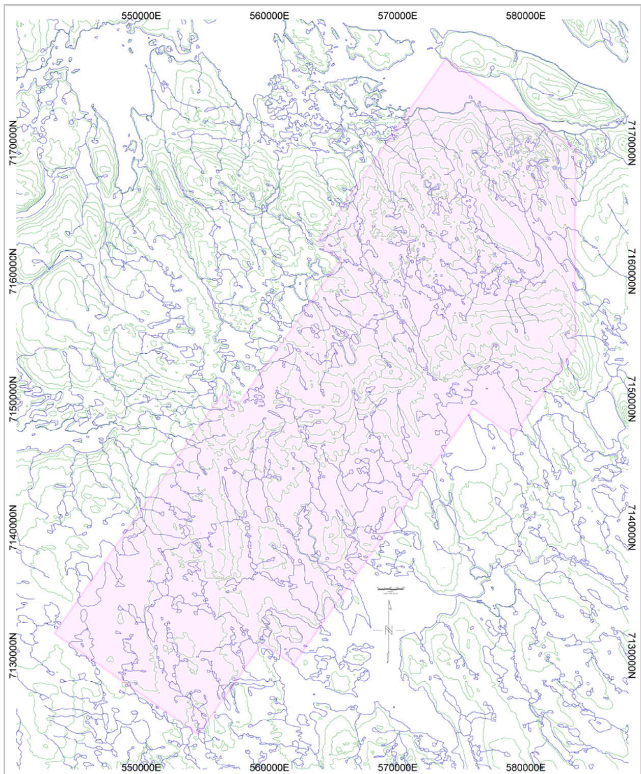
Figure 10: Planned Airborne Gravity Gradiometer Survey. The limits of the survey are outlined by the overlying light magenta polygon. The fixed wing survey aircraft will fly at approximately 90 to 100 m altitude above the ground surface.
