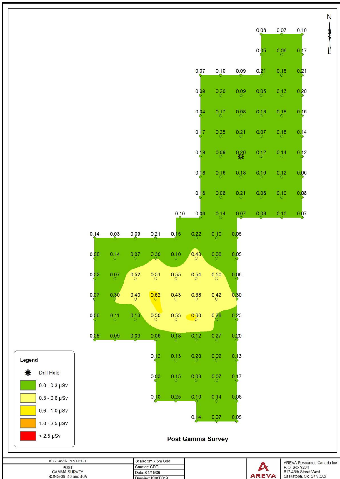
Figure 9.12 Gamma Surveys BONG-39,-40,-40A
