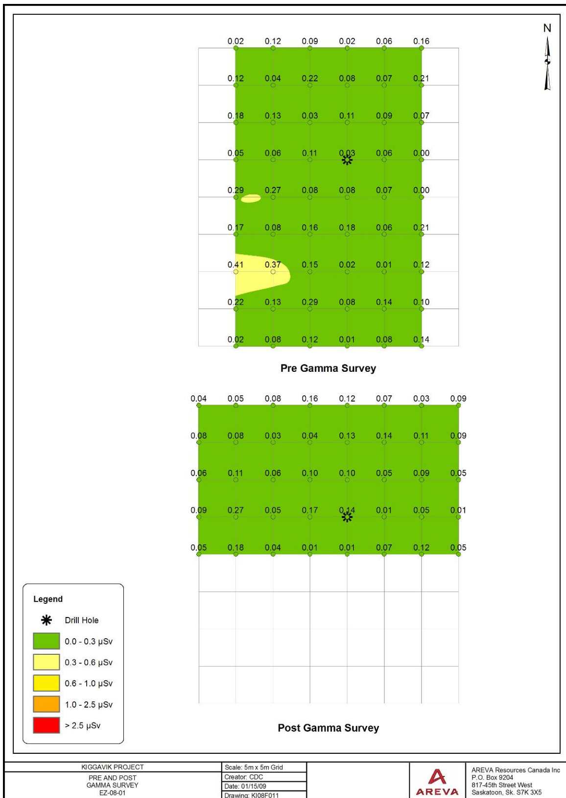
Figure 9.13 Gamma Surveys EZ-08-01
