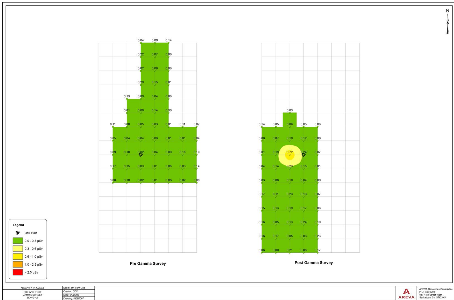
Figure 9.8 Gamma Surveys BONG-42
