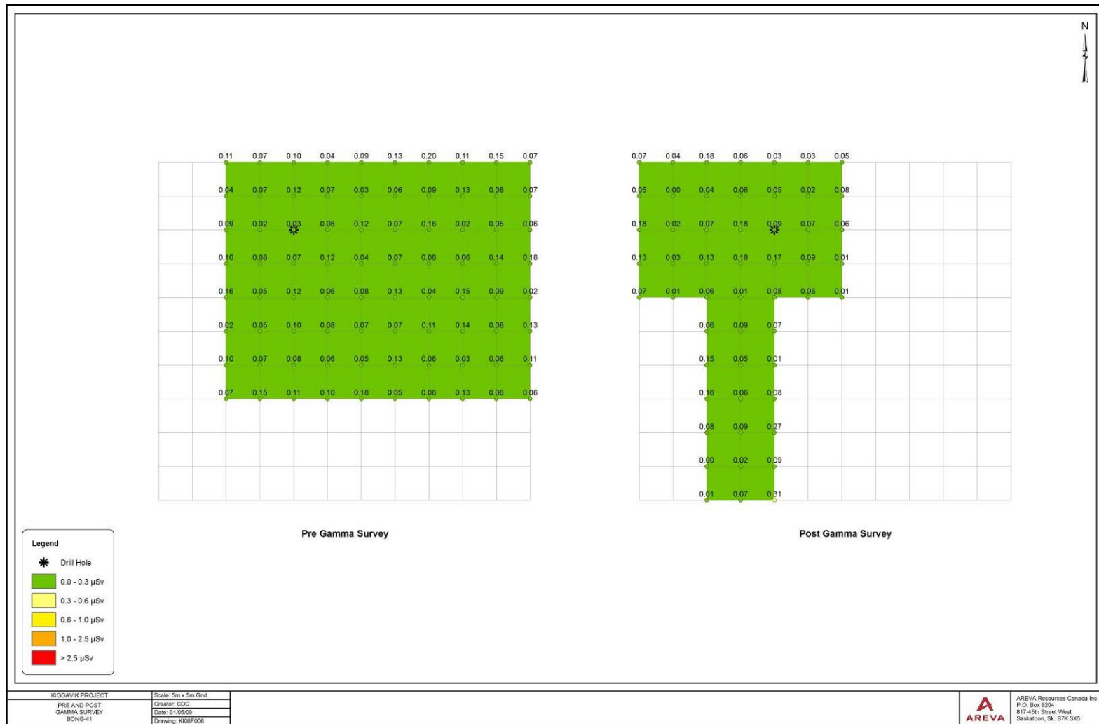
Figure 9.7 Gamma Surveys BONG-41
