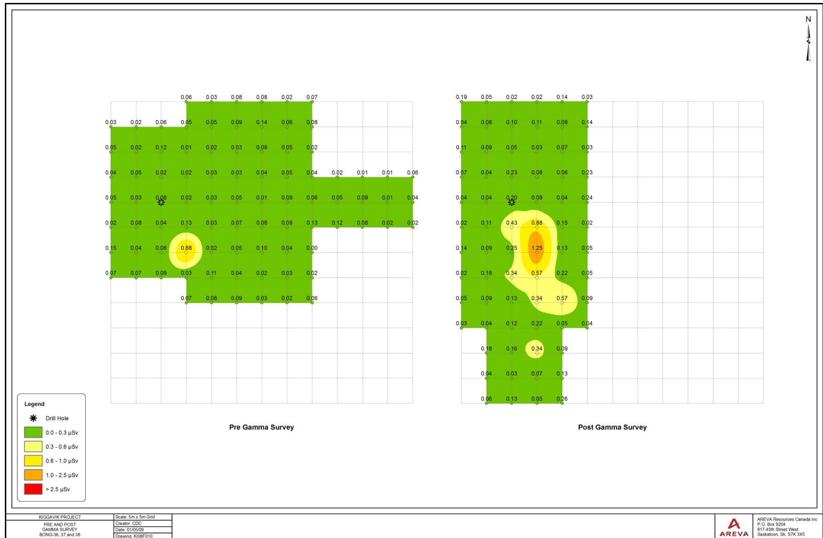
Figure 9.11 Gamma Surveys BONG-36,-37,-38
