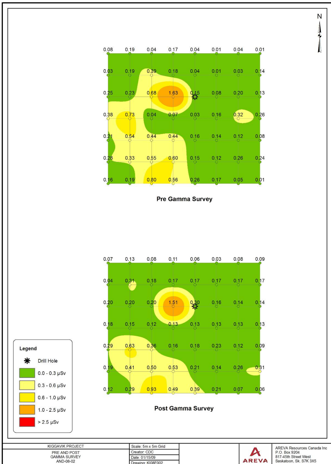
Figure 9.3 Gamma Surveys AND-08-02
