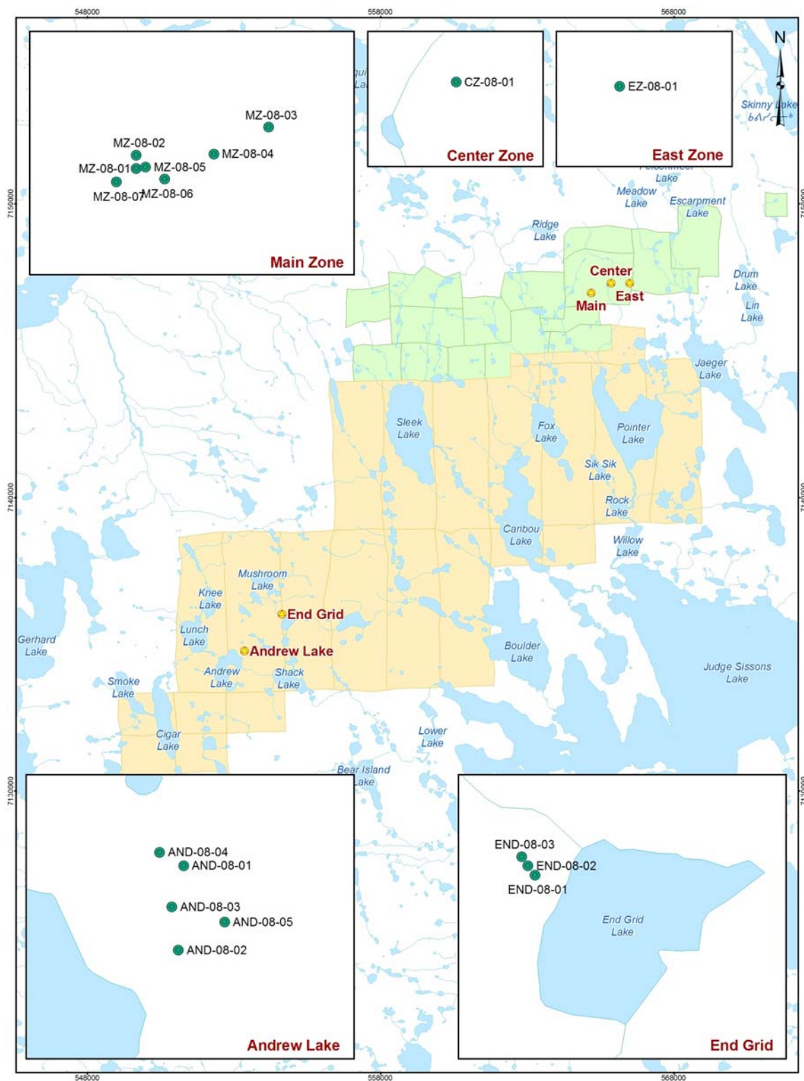
Figure 9.1 2008 Drill Hole Locations
