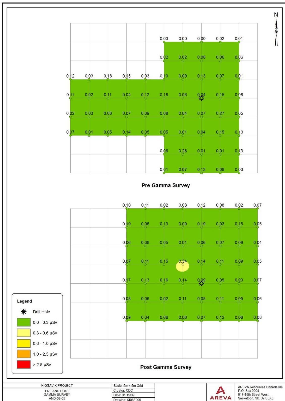
Figure 9.6 Gamma Surveys AND-08-05
