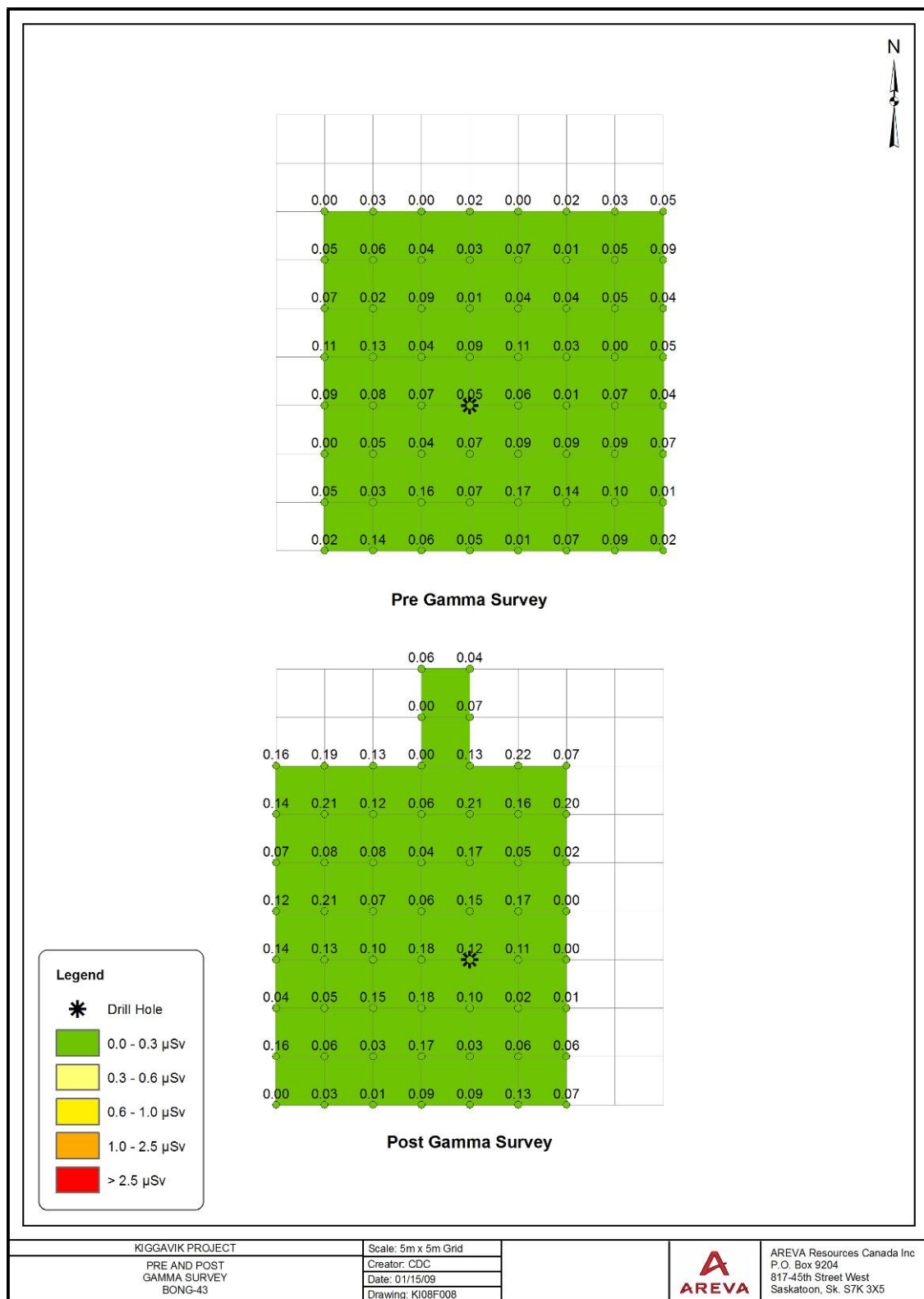
Figure 9.9 Gamma Surveys BONG-43
