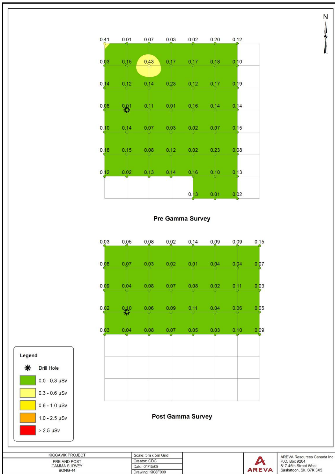
Figure 9.10 Gamma Surveys BONG-44
