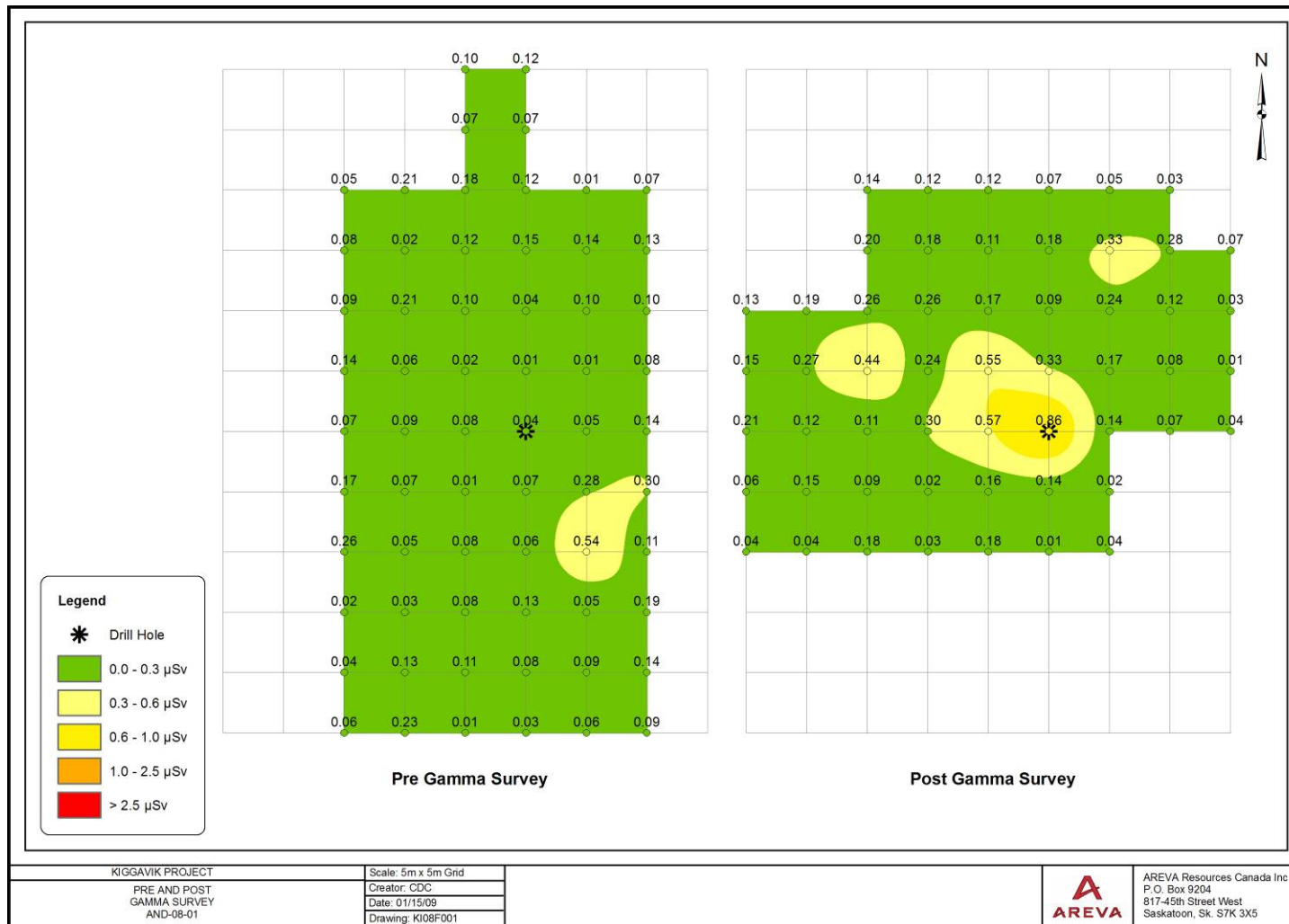
Figure 9.2 Gamma Surveys AND-08-01
