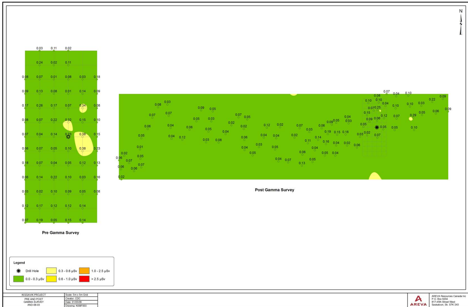
Figure 9.4 Gamma Surveys AND-08-03
