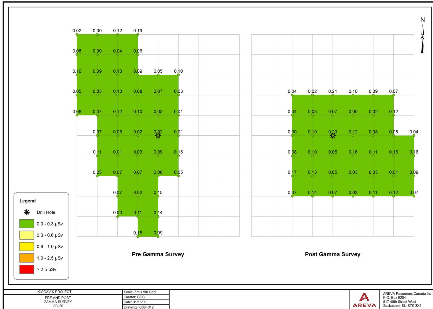
Figure 9.14 Gamma Surveys GG-20
