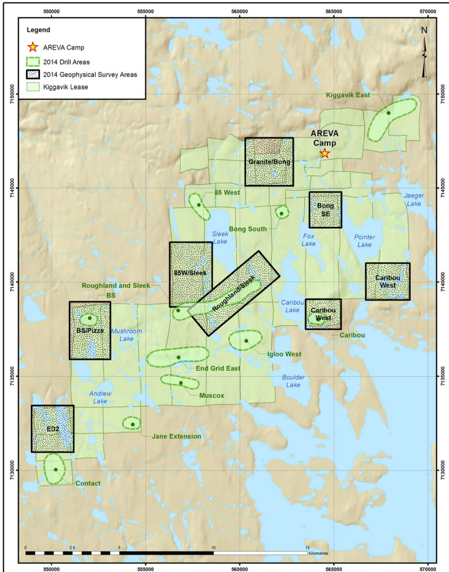
FIGURE 1.0 2014 Geophysical and Drilling Areas
