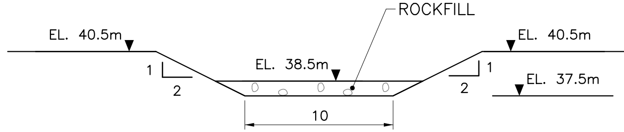
D SECTION - SPILLWAY - STEENSBY INLET PORT SCALE: 1:250
