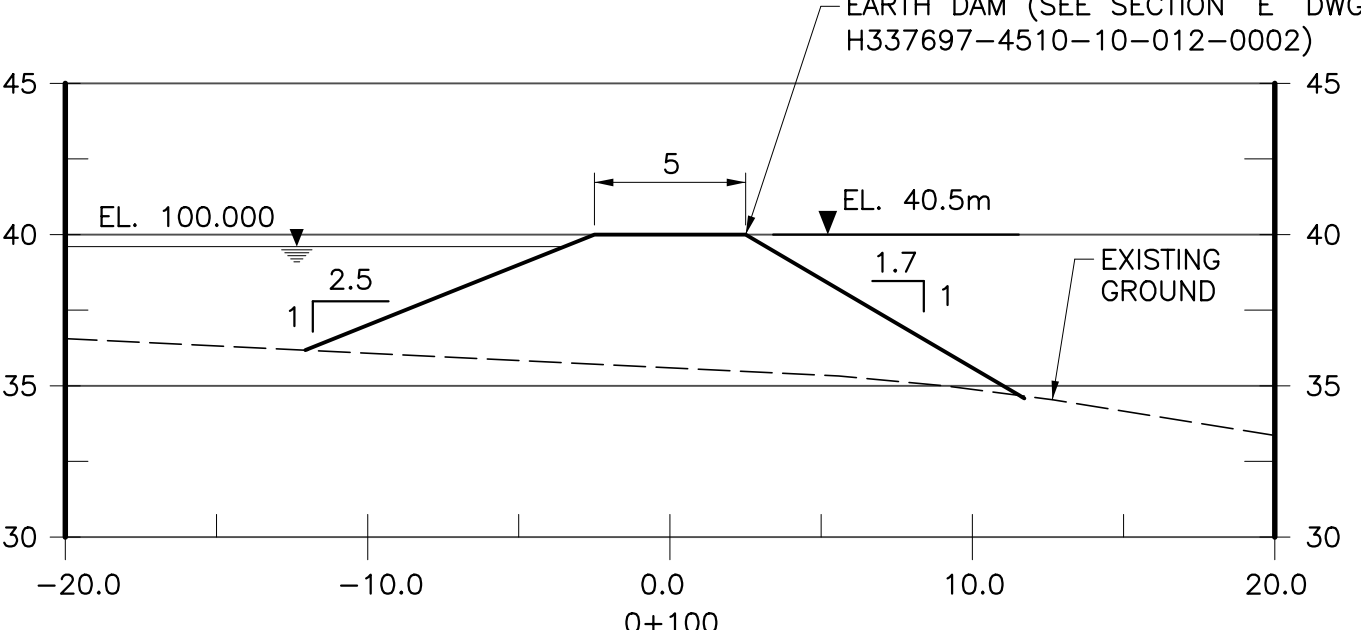
A SECTION - DAM - STEENSBY INLET PORT SCALE: 1:250
