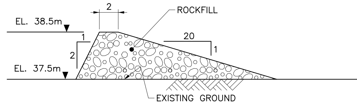
C SECTION - SPILLWAY - STEENSBY INLET PORT SCALE: 1:250
