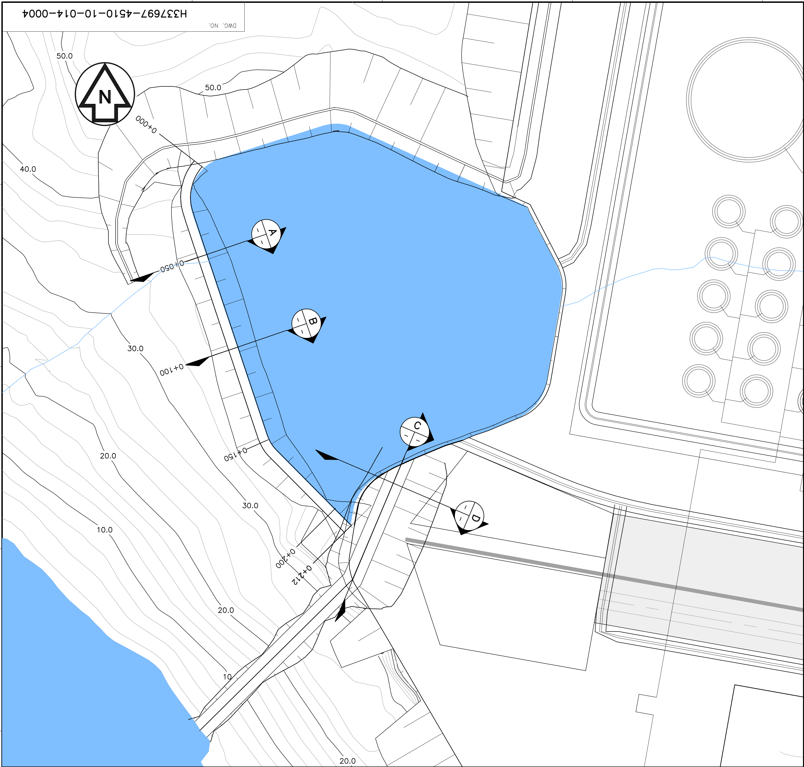
1 PLAN - POND DAM STEENSBY INLET PORT SCALE: 1:1000
