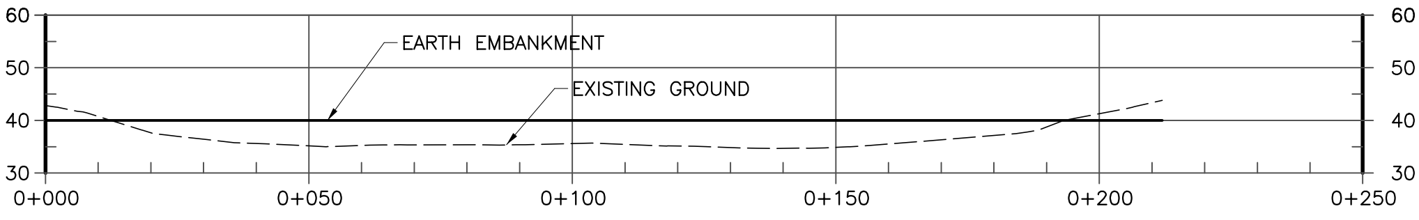
2 PROFILE - DAM - STEENSBY INLET PORT SCALE: 1:1000
