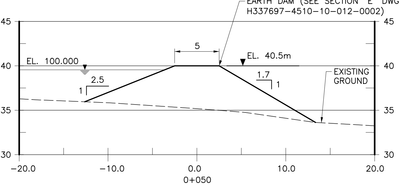
B SECTION - DAM - STEENSBY INLET PORT SCALE: 1:250
