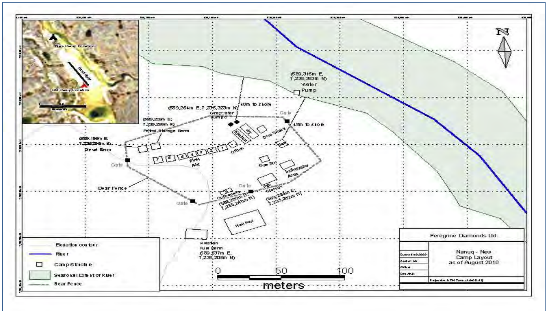
FIGURE 3: Nanuq Camp Layout, Current at August 2010 (Additions for this year: 1 new sleep tent and a bear fence).
