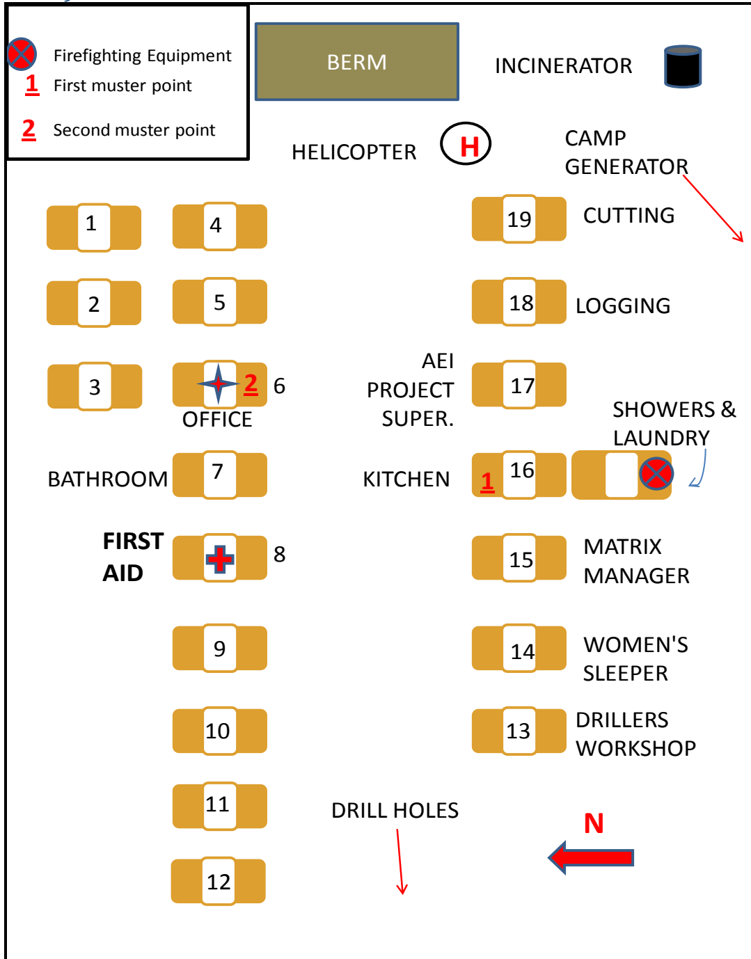
Figure 2: Schematic of Temporary Exploration Camp Layout (not to scale)
