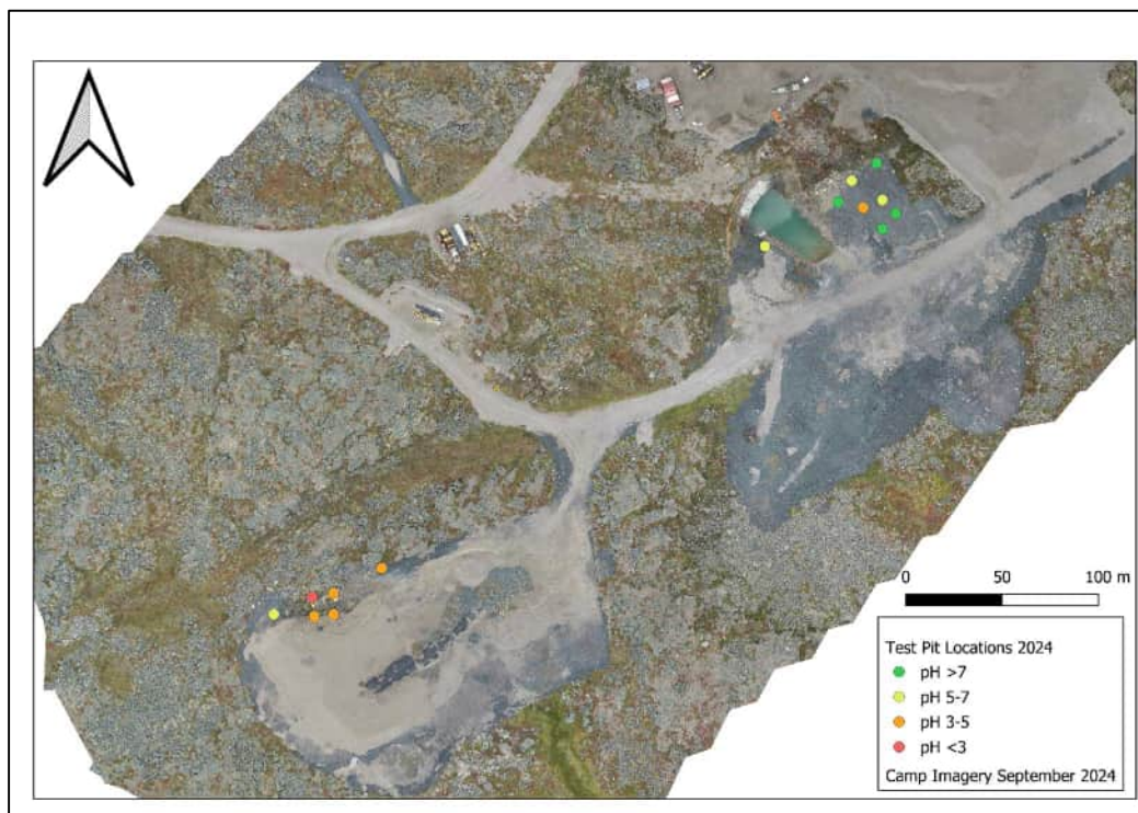
Figure 4. Ulu Gold Project pH test pit locations.
