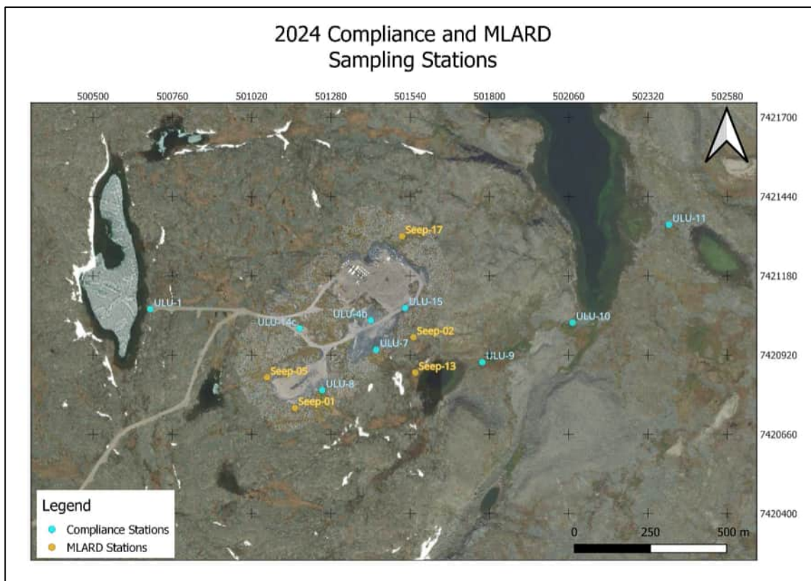
Figure 3. Ulu Gold Project seepage sampling locations.
