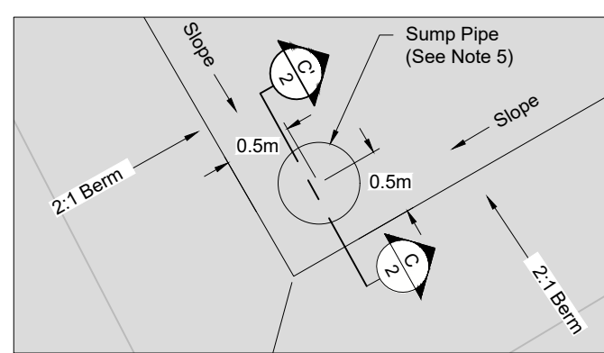
Detail 1 - Typical Sump
