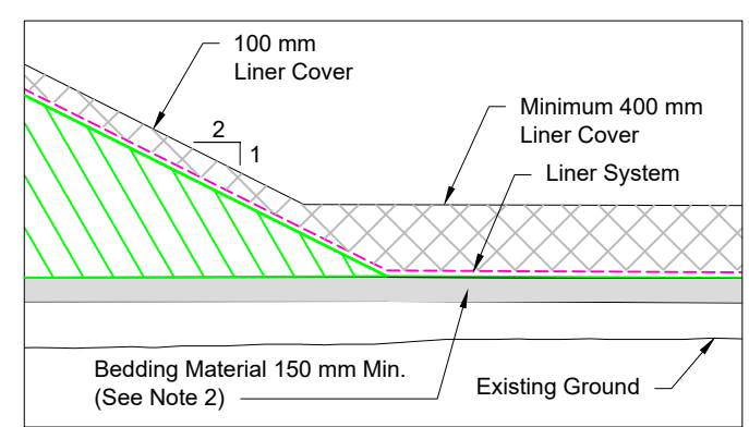
Detail 3 - Liner Cover (See Note 3)
