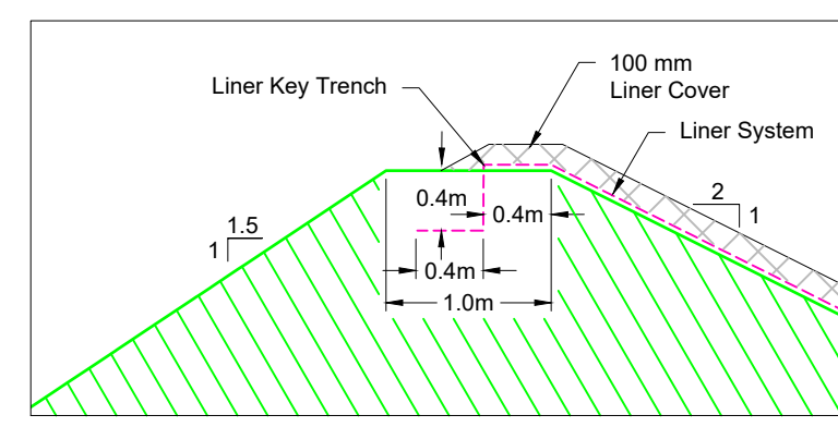
Detail 2 - Liner Tie-In
