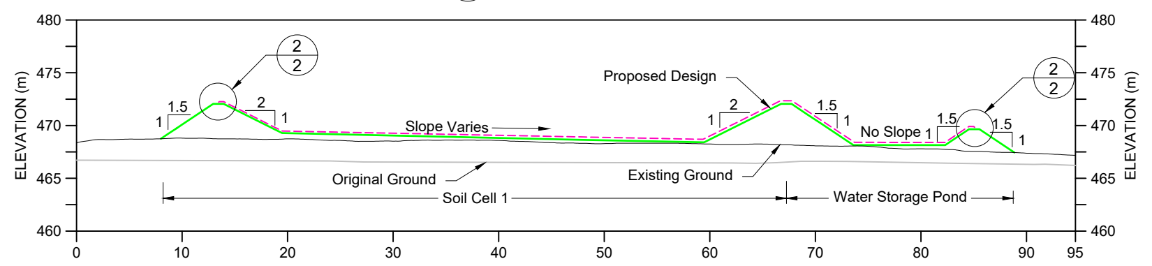
Cross Section B-B'
