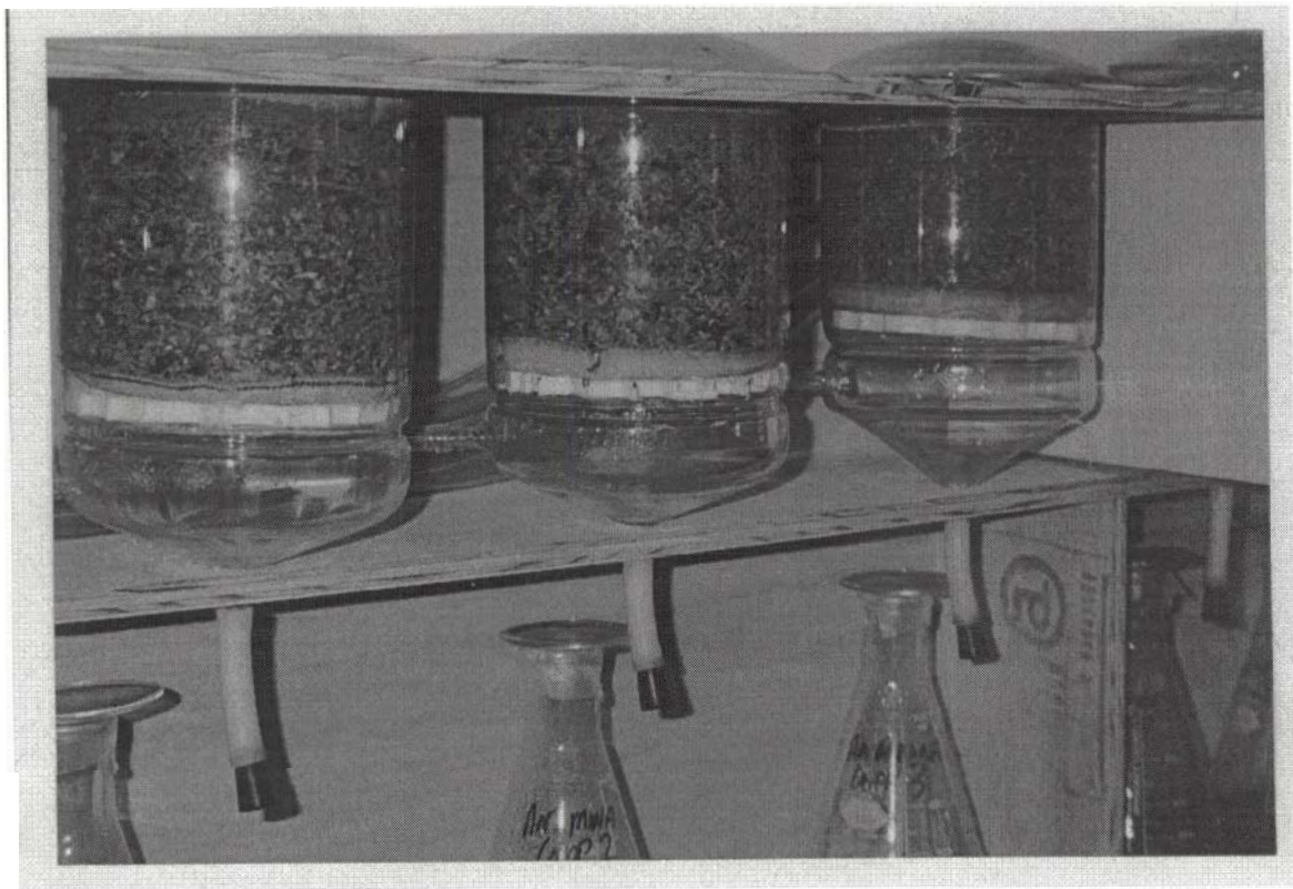
Figure 2 A photograph showing the room-temperature humidity cell setup.
