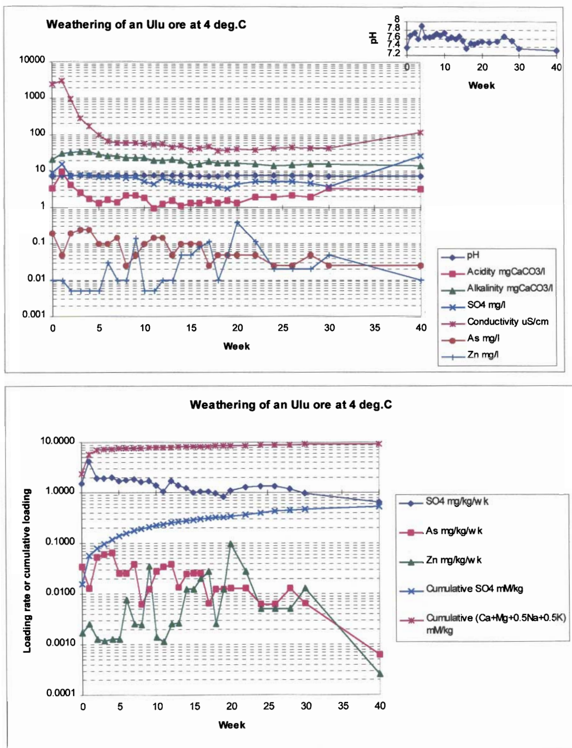
Figure 3 Time series of selected parameters determined during humidity-cell testing of an Ulu ore at 4°C.
