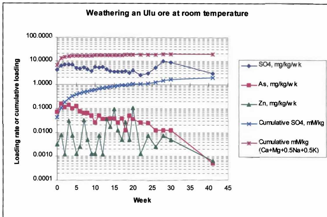
Figure 4 Time series of selected parameters determined during humidity-cell testing of an Ulu ore at room temperature
