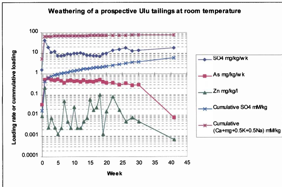
Figure 8 Time series of selected parameters measured or derived in the humidity-cell testing of a prospective Ulu tailings sample at room temperature.
