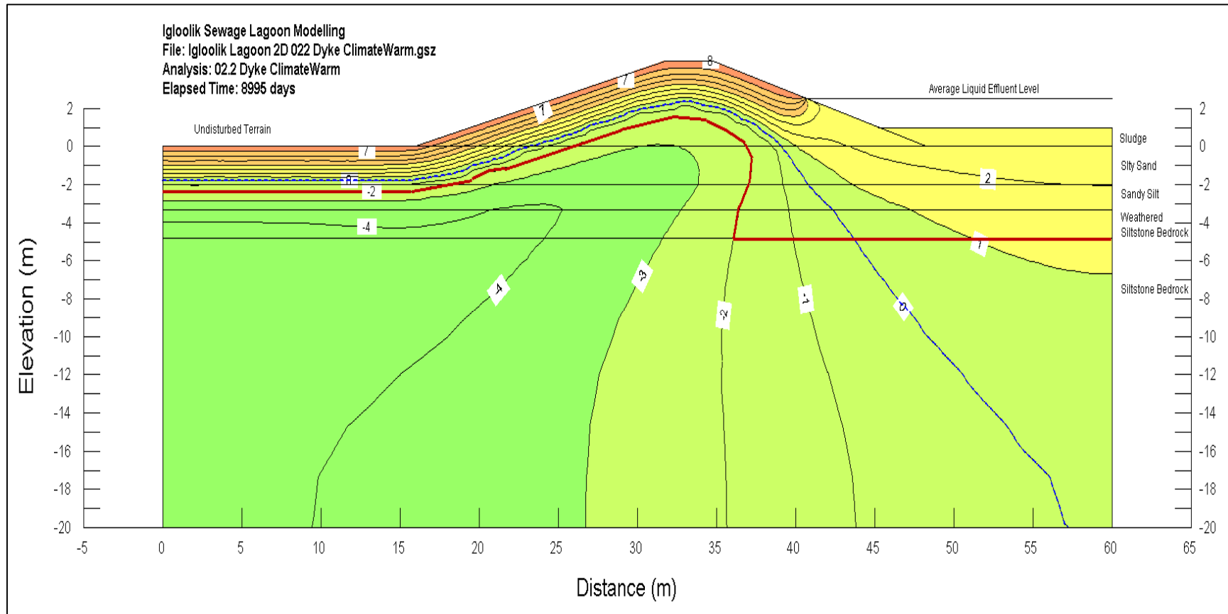
Figure 4-3. Cross-section of containment structure showing ground temperature contours after 20 years.
