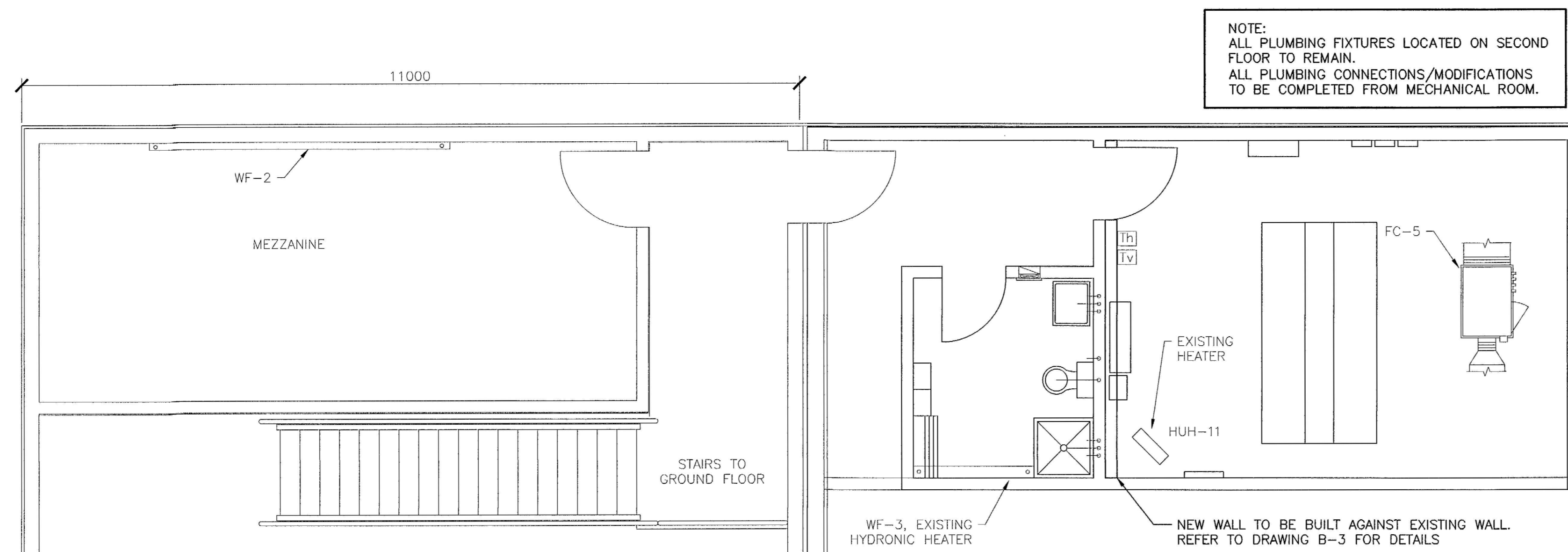
MECHANICAL PLUMBING - MEZZANINE FLOOR PLAN 1:50
