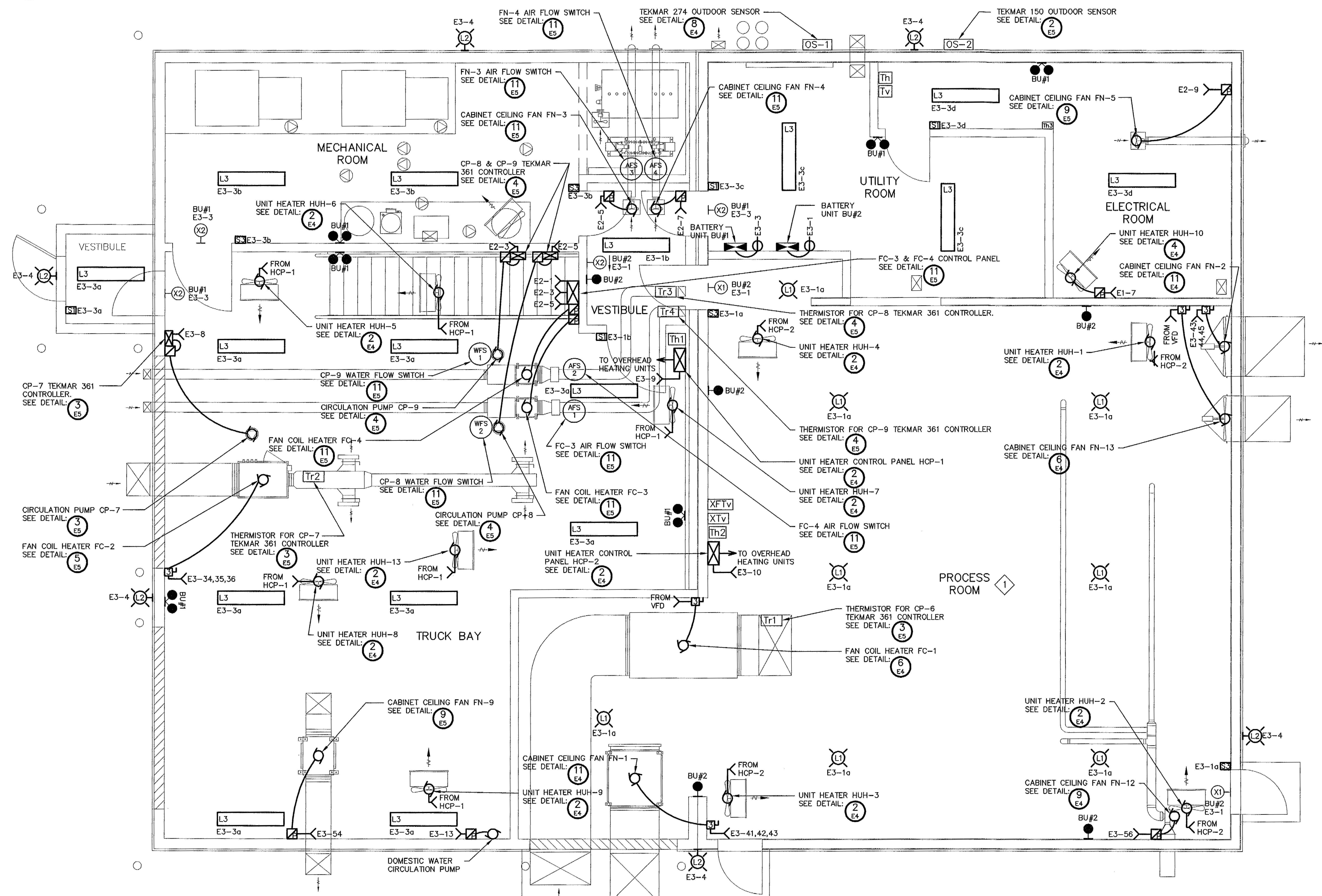
3 ELECTRICAL BUILDING LAYOUT – PROPOSED LOWER LEVEL LIGHTING AND HVAC E9 SCALE 1:50
