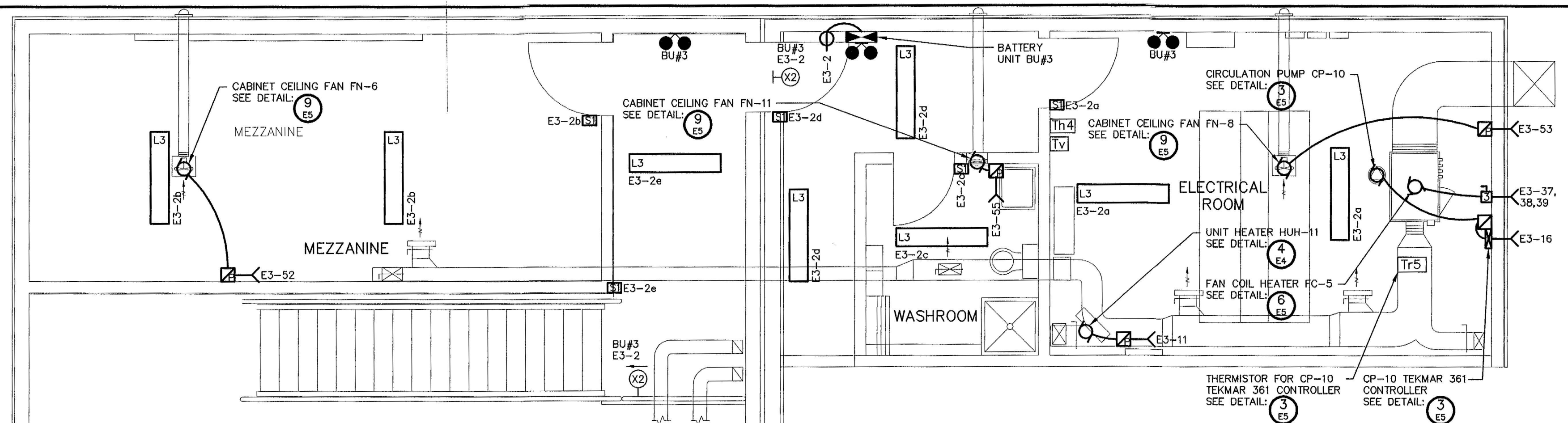
2 ELECTRICAL BUILDING LAYOUT – PROPOSED UPPER LEVEL LIGHTING AND HVAC E9 SCALE 1:50
