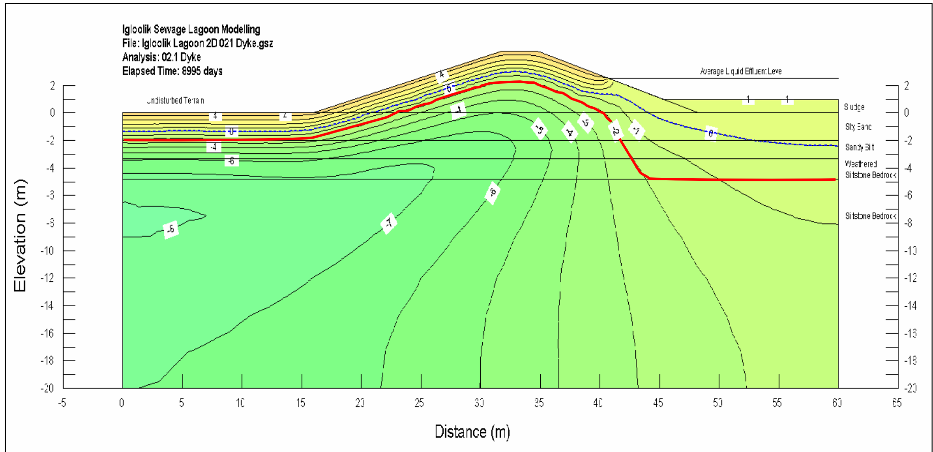
Figure 4-2. Cross-section of containment structure showing ground temperature contours after 20 years. No climate warming effects are included. The red contour line represents the -2 °C isotherm above the bedrock elevation and the weathered/unweathered bedrock interface.
