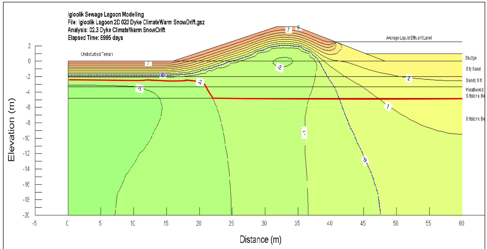
Figure 4-4. Cross-section of containment structure showing ground temperature contours after 20 years. Climate warming and snow drifting effects are included. The red contour line represents the -2 °C isotherm above the bedrock elevation and the weathered/unweathered bedrock interface.
