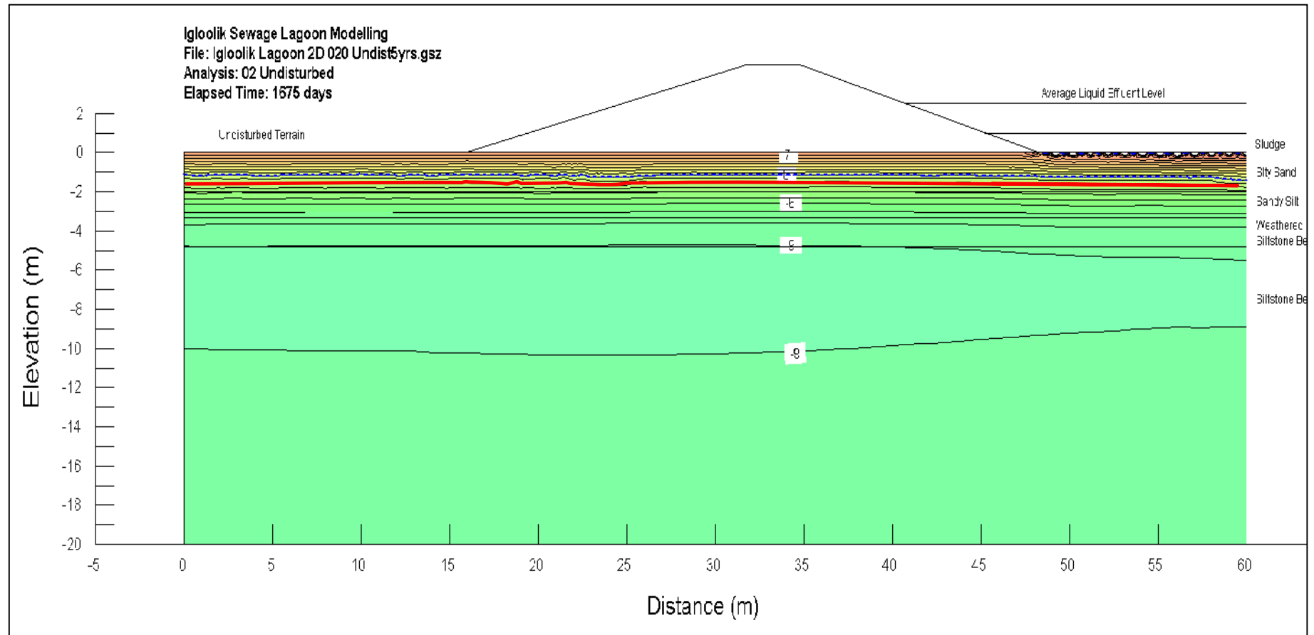
Figure 4-1. Cross-section of berm sub-grade showing ground temperature contours at maximum thaw at 4.59 years, prior to construction of the containment structure. The red contour line represents the -2 °C isotherm.
