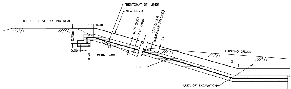
LINER DETAIL 1:50
