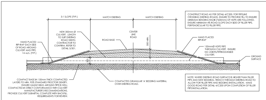
5 TYPICAL SECTION: ROAD OVER NEW PIPELINE C101 1:40
