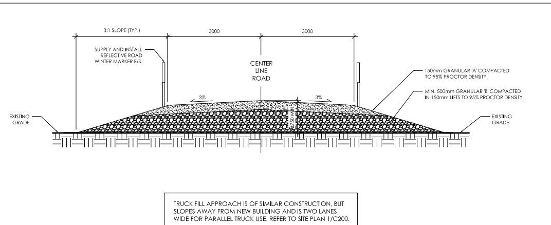
2 TYPICAL ROAD SECTION 1:40
